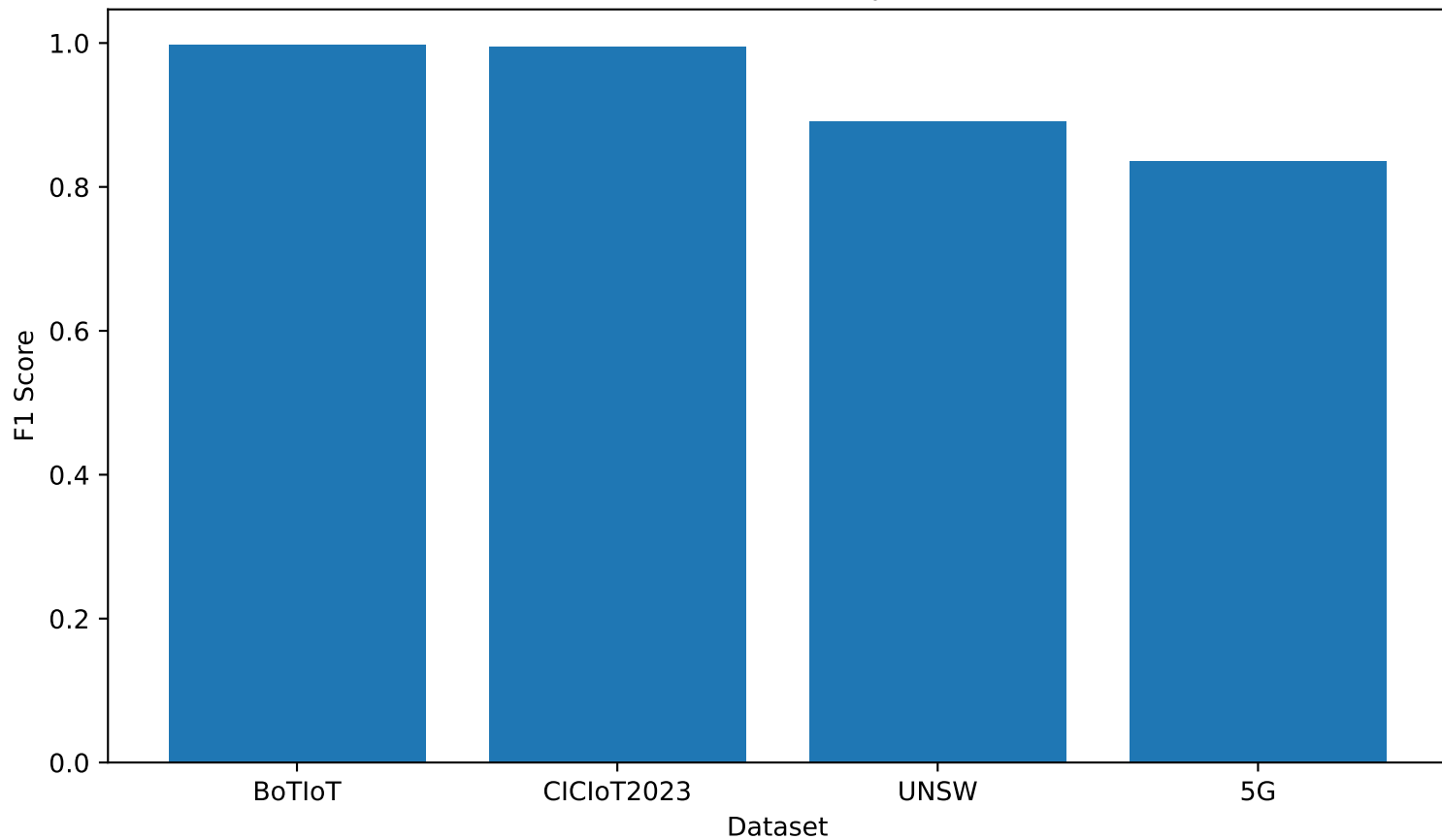
Domain-wise Evaluation of Proposed Ensemble-4
