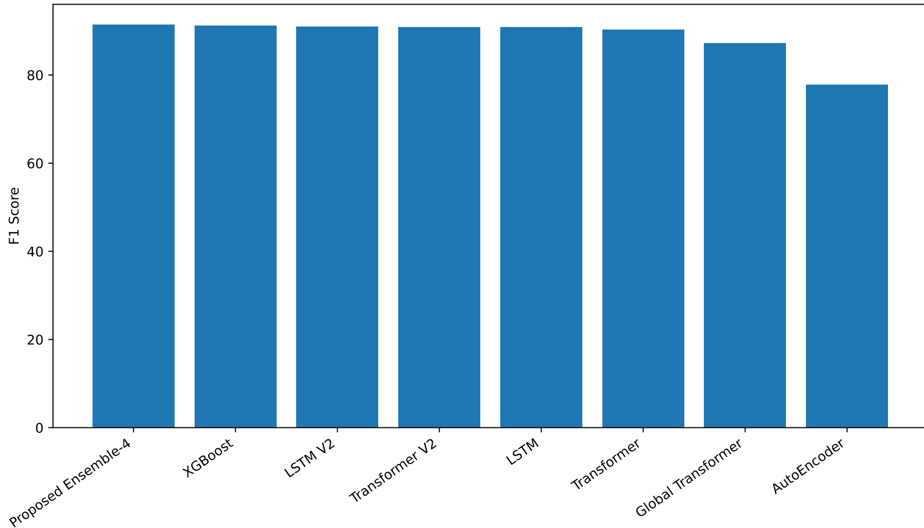
Model Comparison on Heterogeneous Dataset
