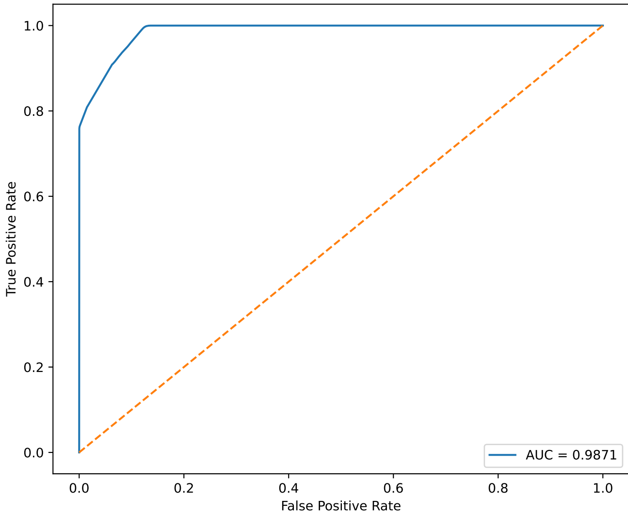
ROC Curve - Proposed Ensemble-4
