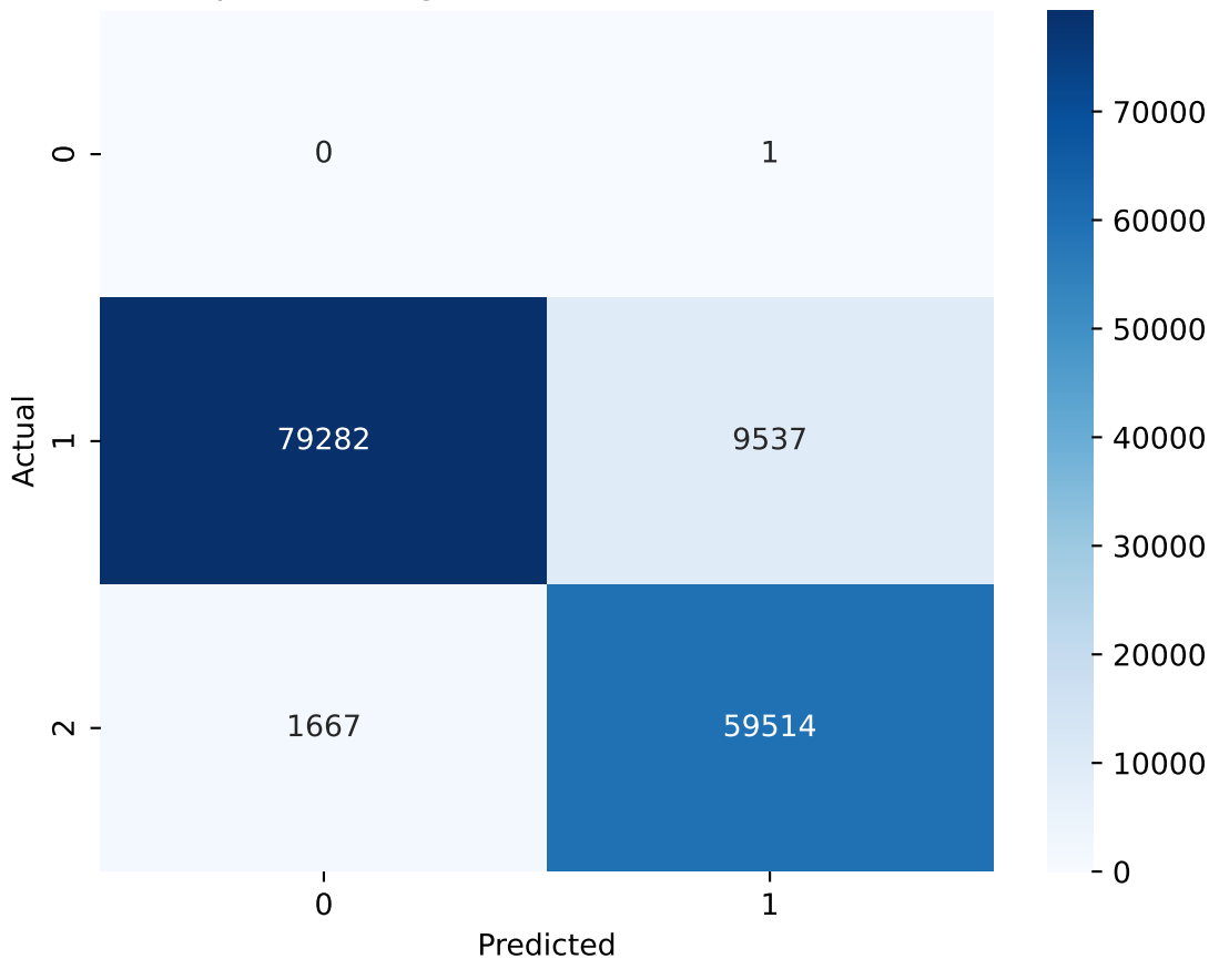
Proper Stacking Ensemble Confusion Matrix
