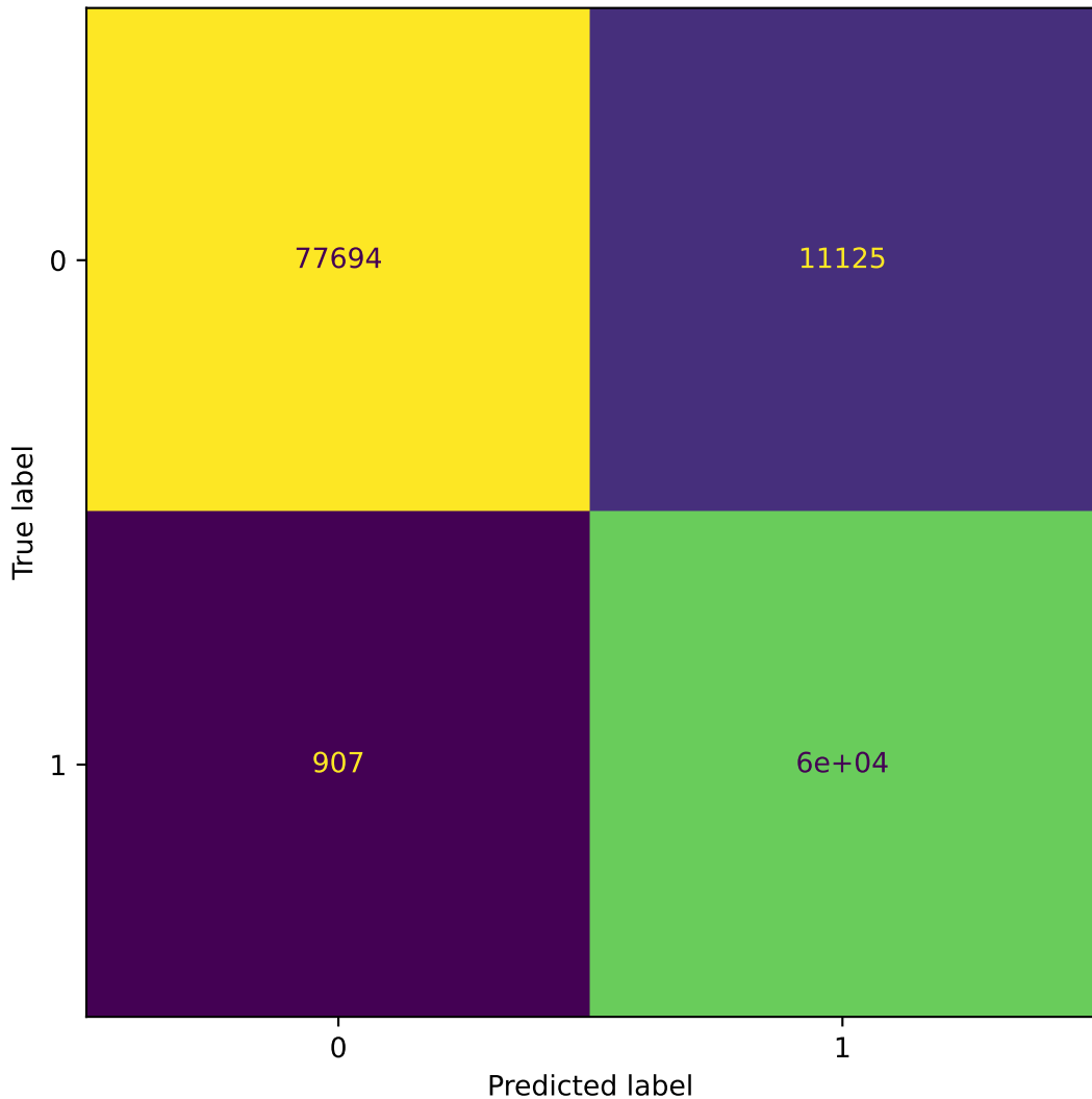
Transformer_V2
