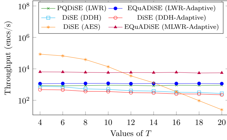
Figure 4: Throughput in DiSE, PQDiSE, EQuADiSE
