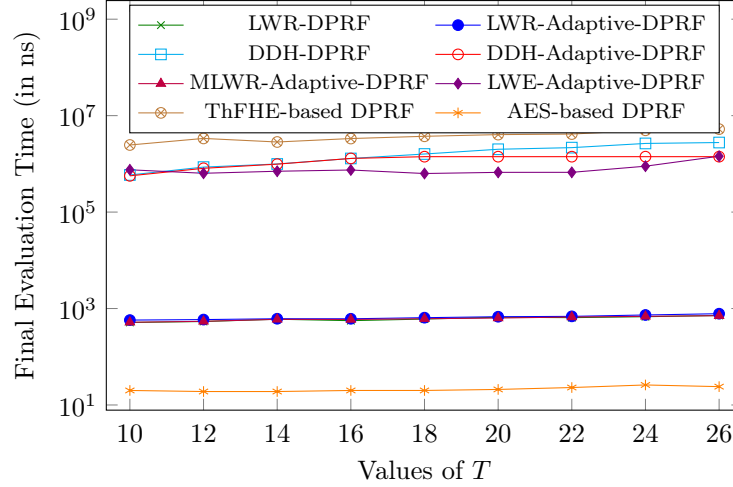
Figure 2: Final evaluation time of (\frac{T}{2}, T) -DPRFs
