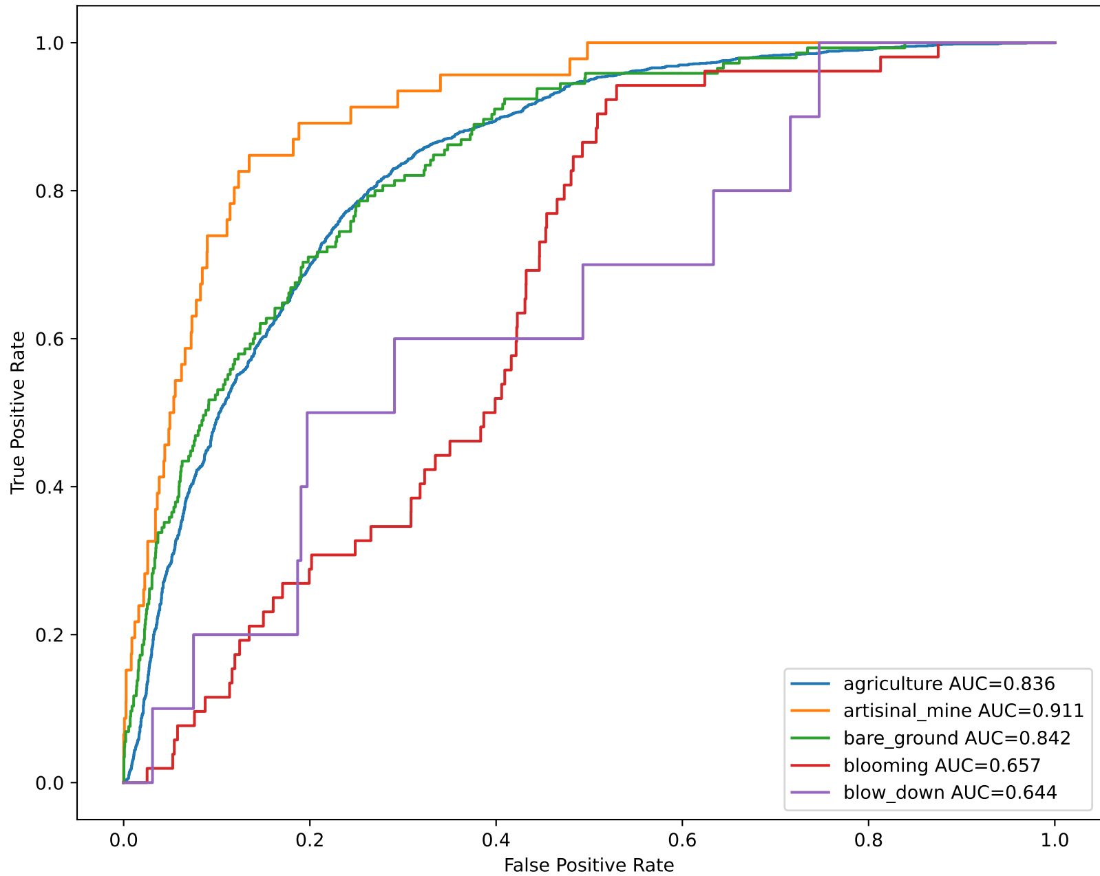
Figure 2.3: ROC Curves for Custom CNN
