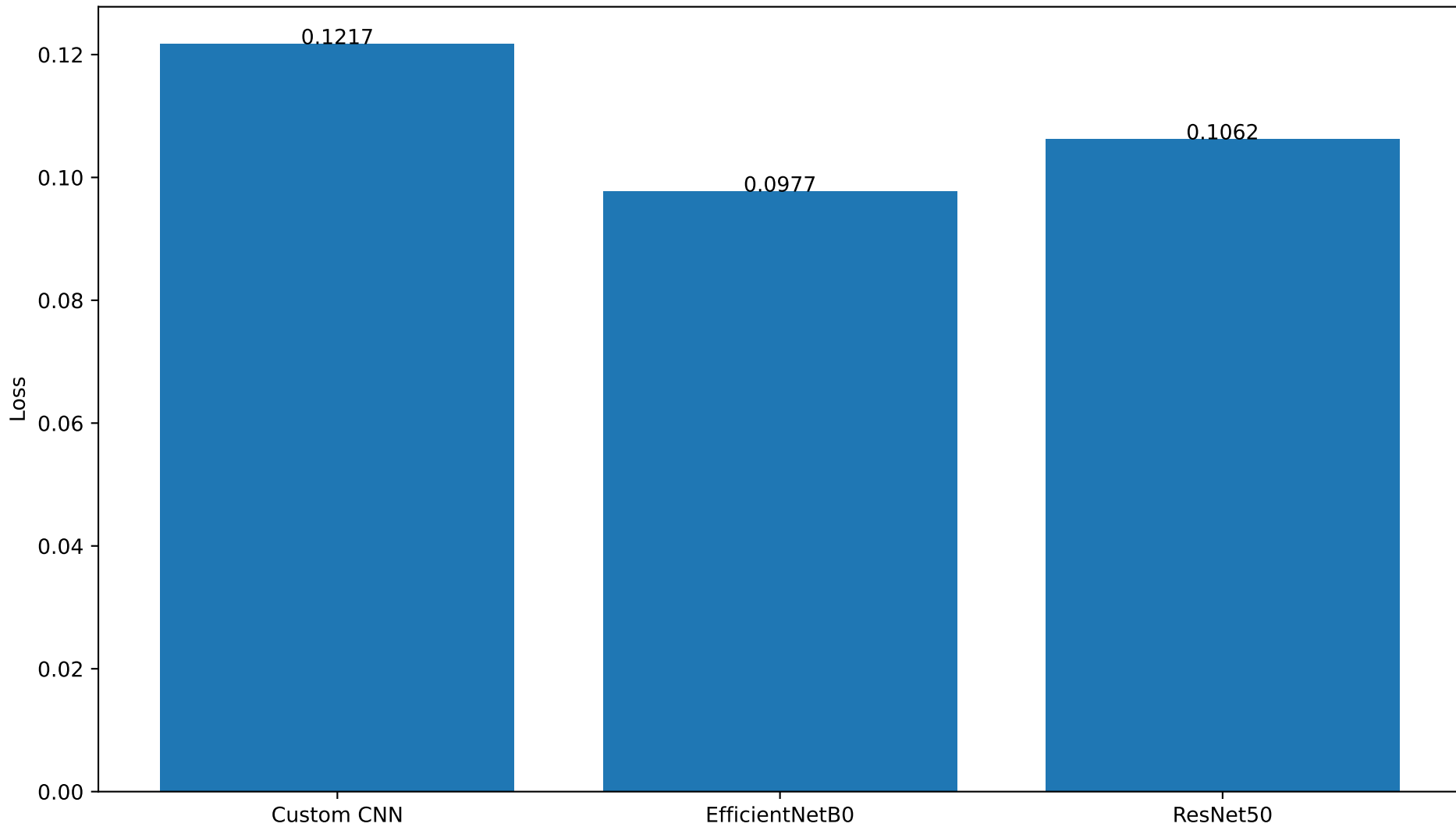
Figure 5.2 Model Loss Comparison
