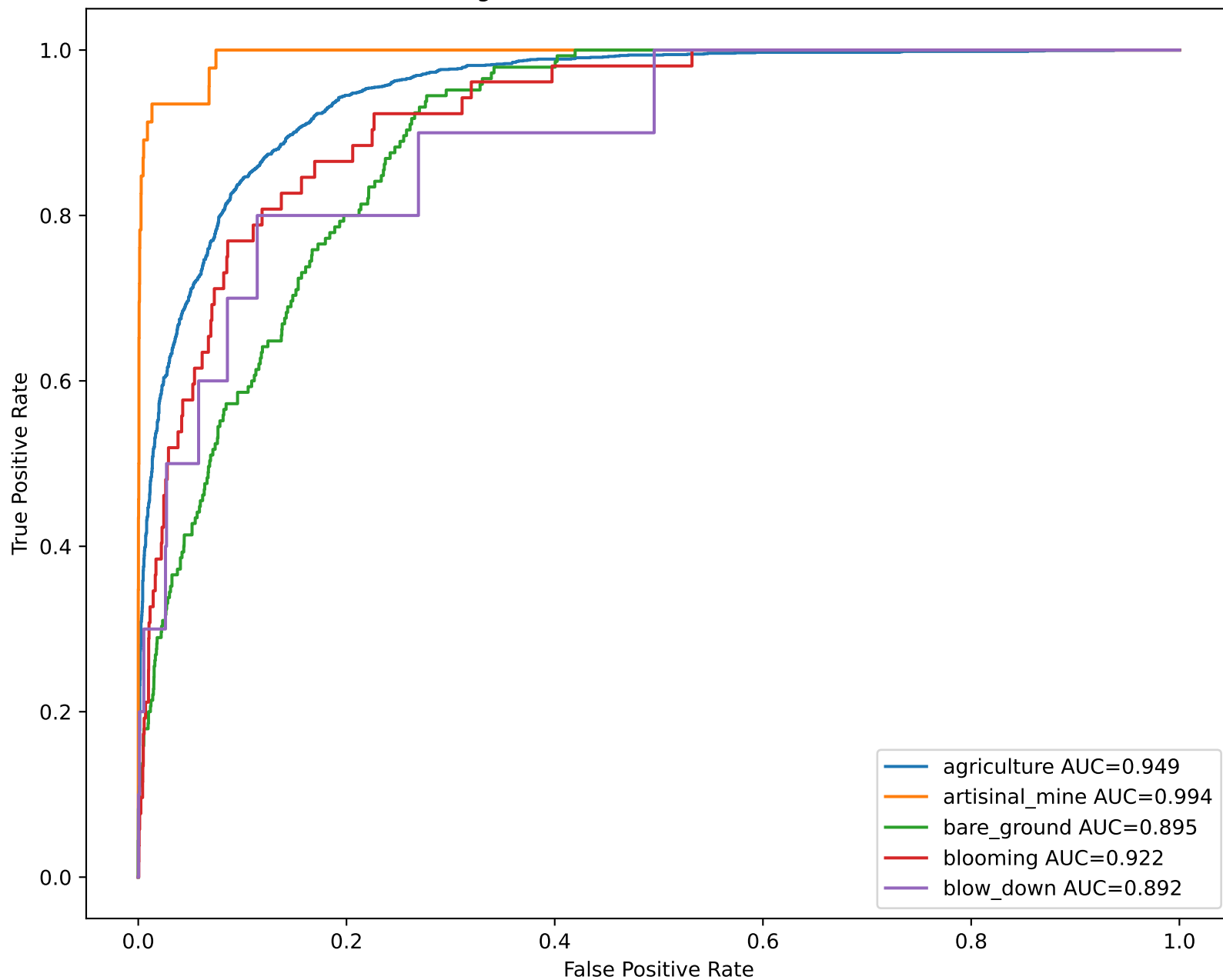
Figure 4.3 ResNet50 ROC Curves
