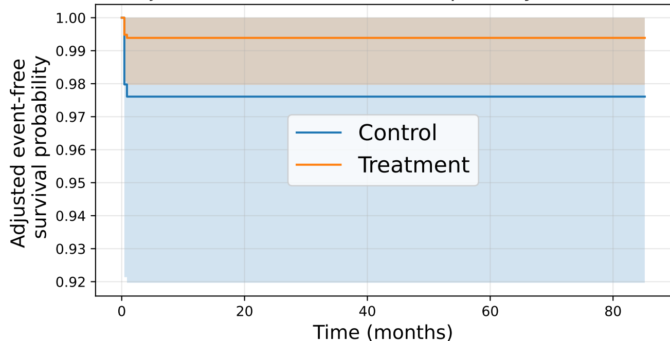
Adjusted Survival Curves: Respiratory disorders
