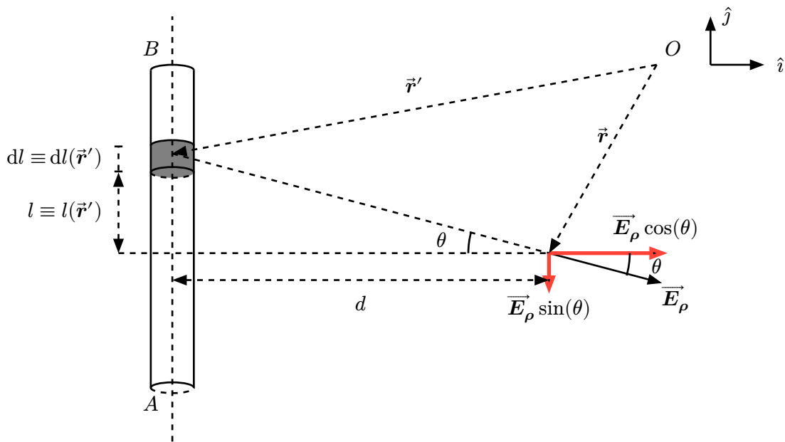
Figure 1: The figure illustrates a rod of finite length \overline{AB} and negligible thickness with a charge density function (per unit length) \rho . An infinitesimally thin slice of the rod at position \vec{r}' w.r.t the origin O is highlighted in grey. This highlighted slice of the rod is of thickness dl and l units away from the center of the rod. The components of the electric field along directions \hat{i} and \hat{j} at a position \vec{r} which is d units away from the center of the rod has been highlighted in red.
