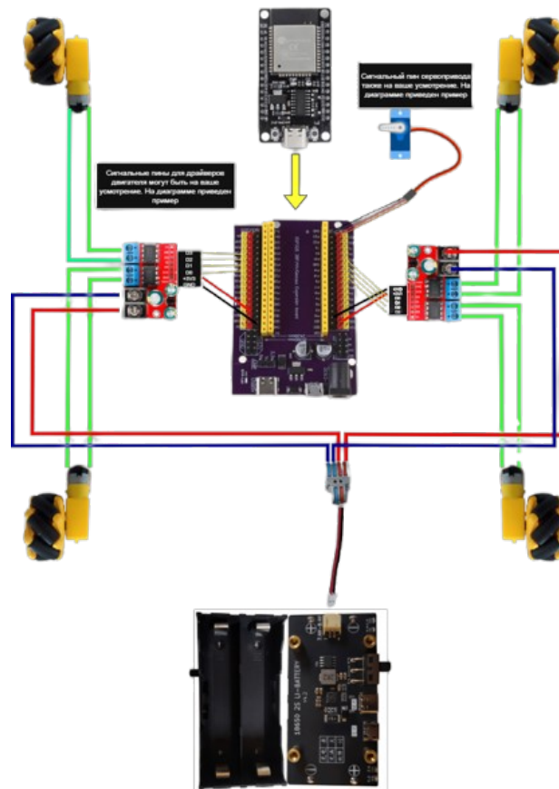
Figure 1: Assemble Scheme
