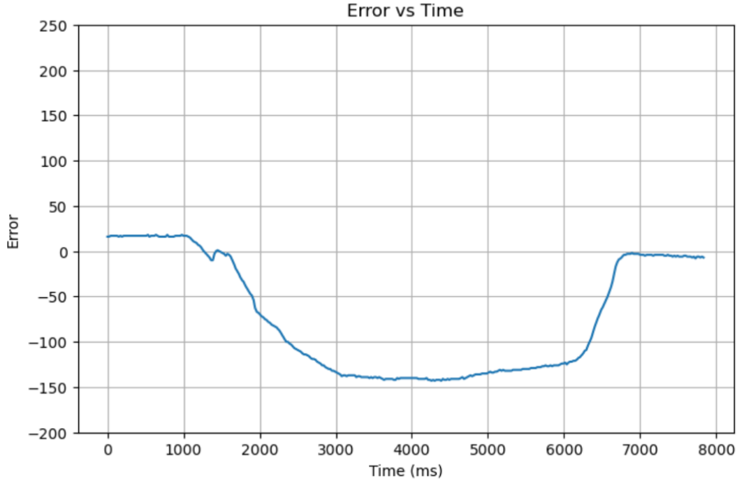
Figure 8: Full PID control
