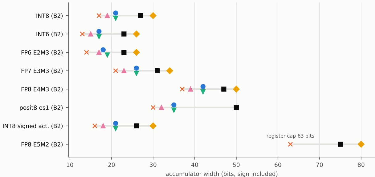
ResNet18, uniform register sat. w < W ; derived widths on ImageNet screen-1k (development evidence)
