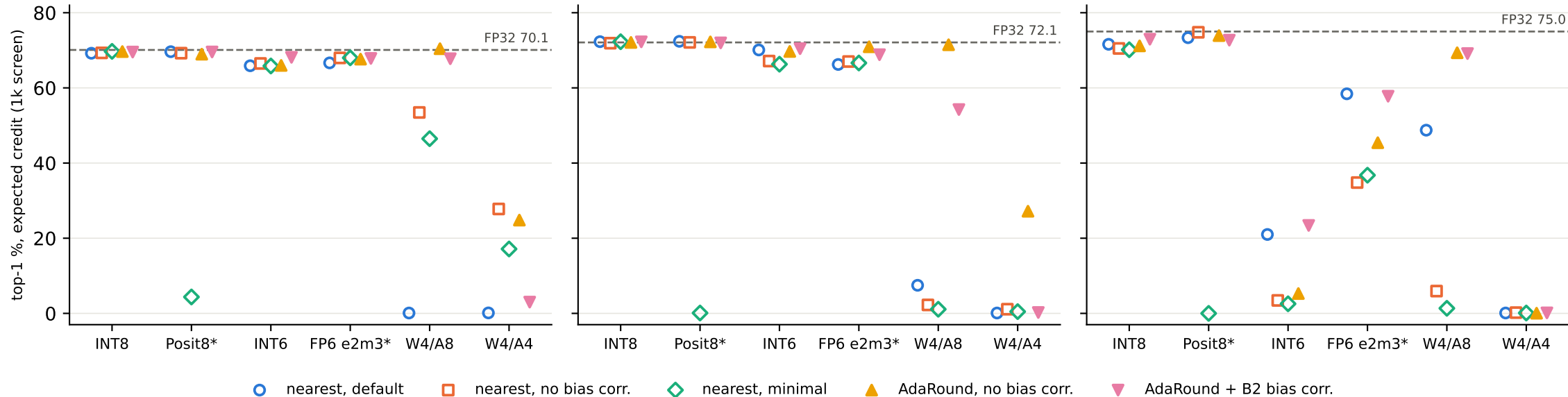
ResNet18
