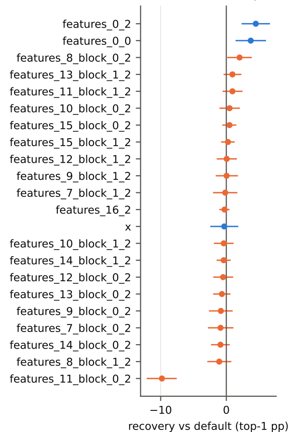
FP6 E2M3: one node kept FP32
