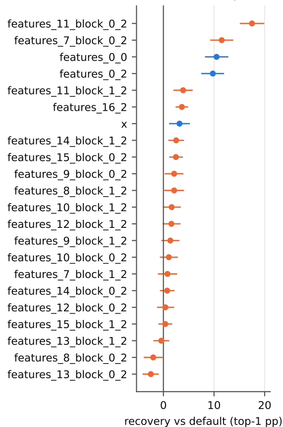
INT6: one node kept FP32
