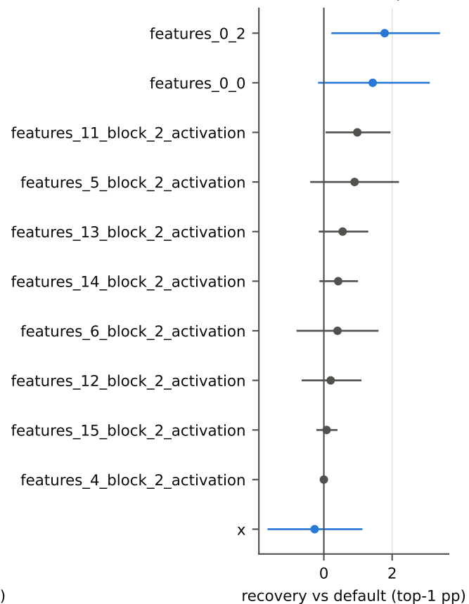
INT8: one node kept FP32
