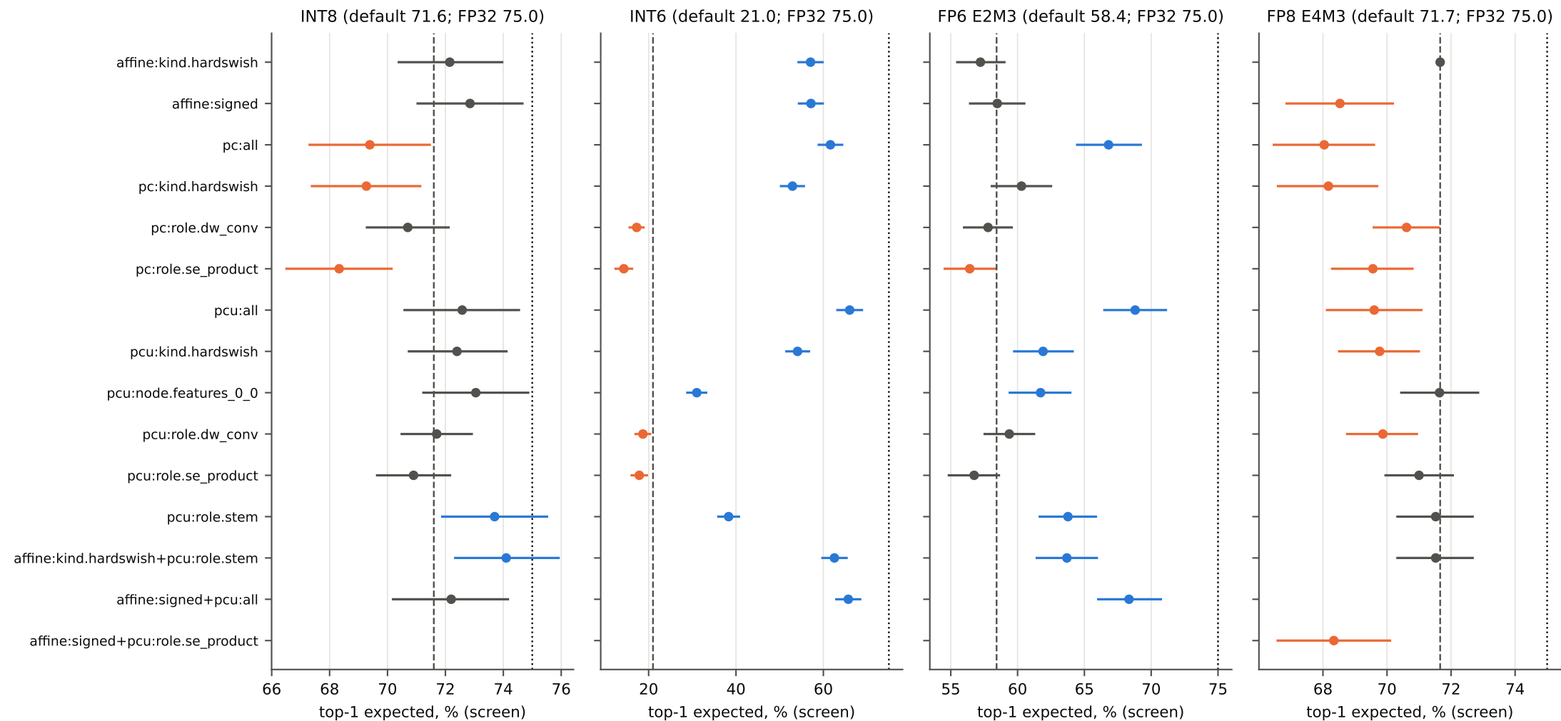
MobileNetV3-L uniform-precision repairs (dashed: frozen default, dotted: FP32; blue/orange: 95 % CI above/below default)
