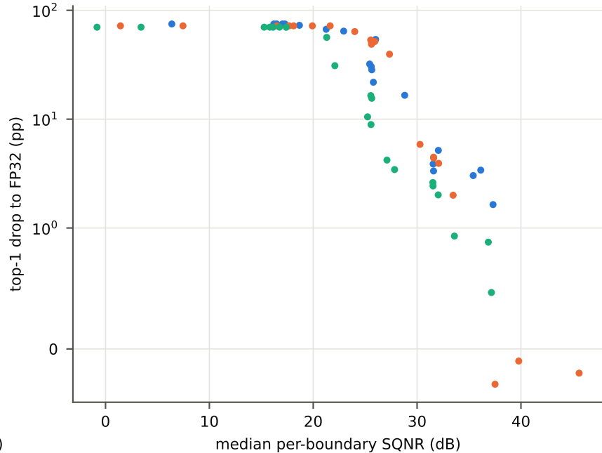
sealed default cells: median SQNR vs top-1 drop (pooled Spearman -0.92)
