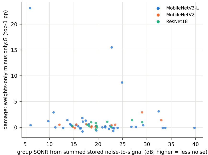
group NSR vs damage (pooled Spearman -0.11, n=63)
