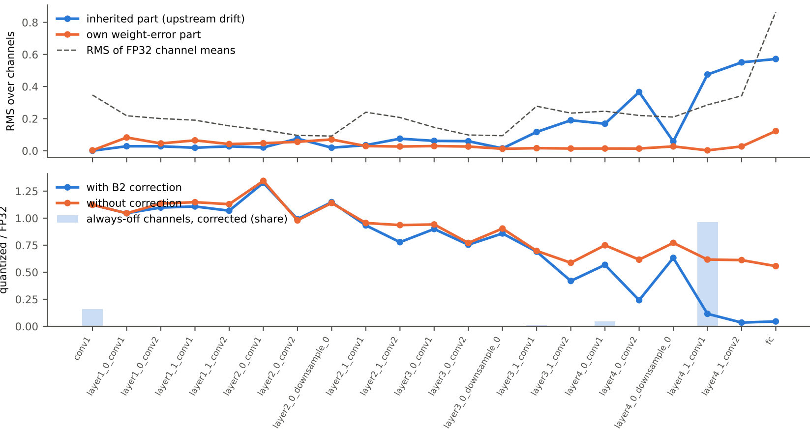
ResNet18, INT4 weights (one scale per layer), FP32 activations: B2 correction per layer
