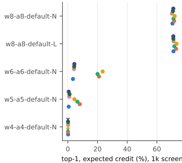
MBv3-L
