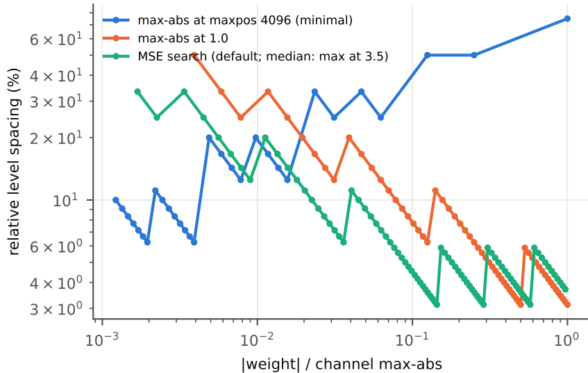
posit8_es1 grid seen by the weights
