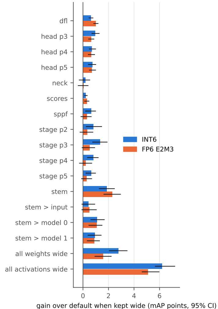
(c) Where the 6-bit loss lives (diagnostic)
