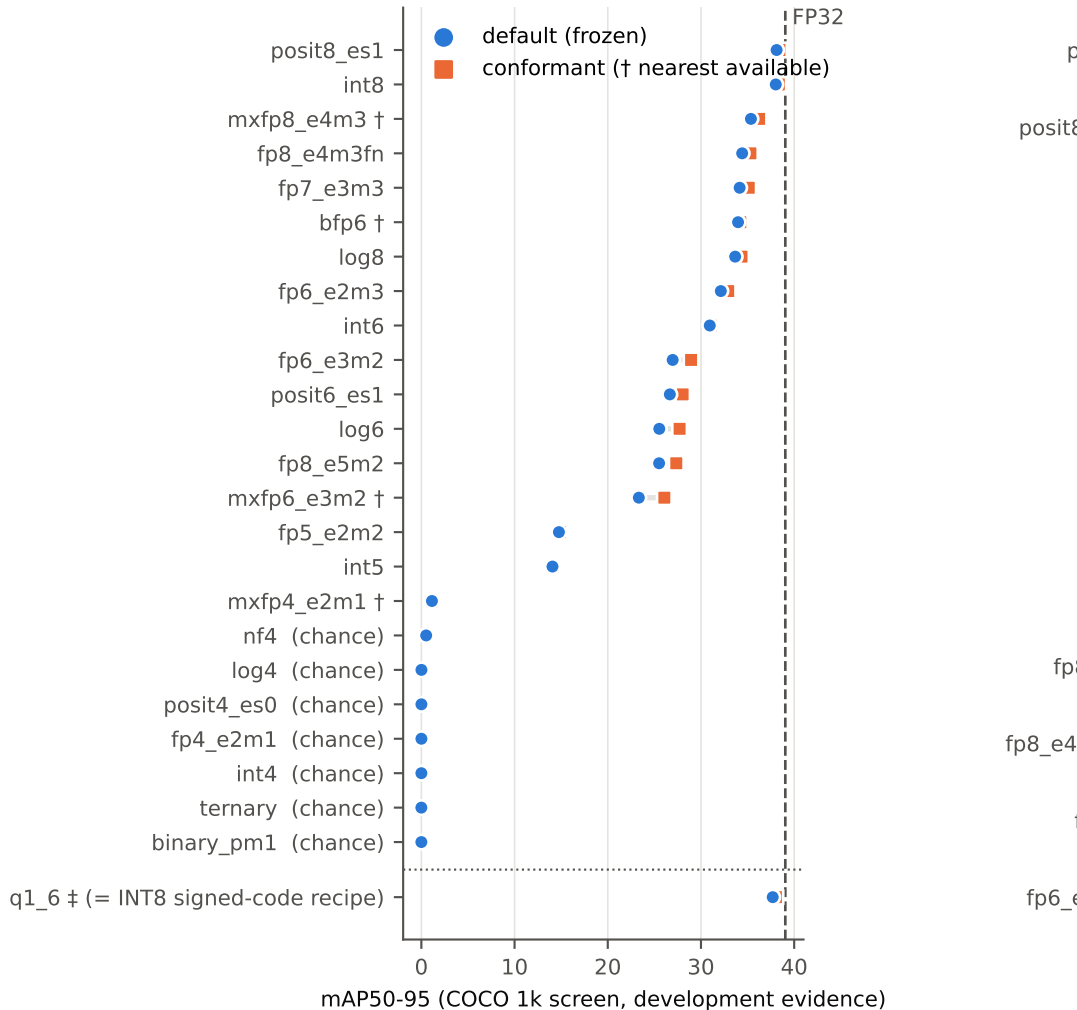
(a) YOLOv8n, 24 formats (‡ set apart)
