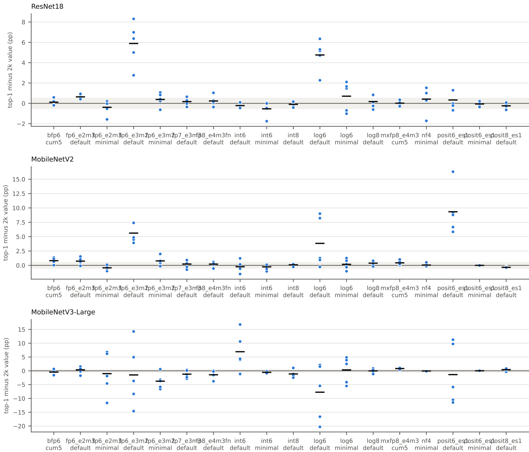
Calibration seeds (5 disjoint 400-image subsets): expected-credit top-1 relative to the 2,000-image calibration; band = \pm \Delta/2 ; bar = seed mean. 1k screen, development evidence.
