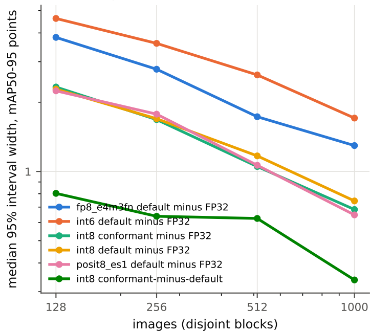
YOLOv8n, paired AP difference
