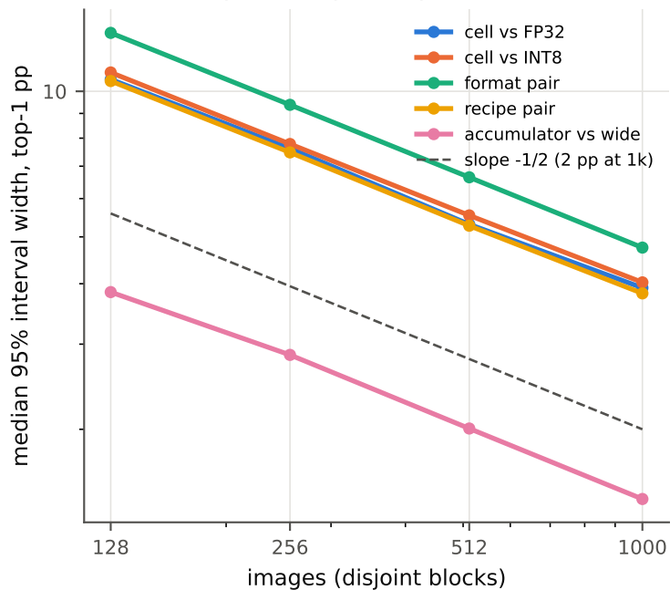
Classifiers, paired top-1 (expected credit)
