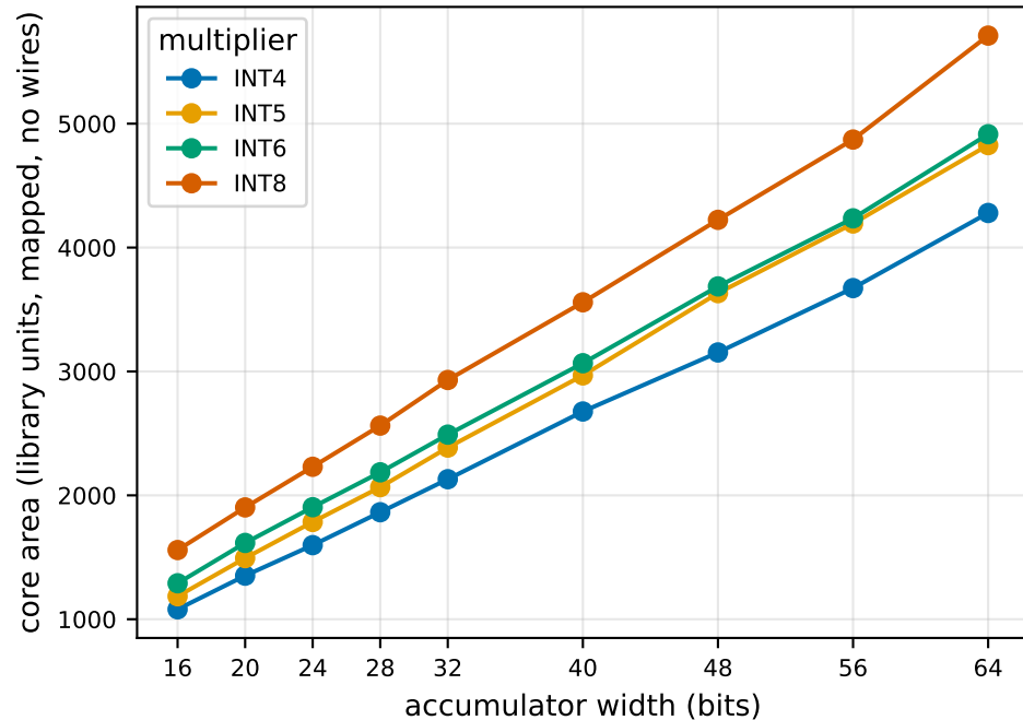
MAC core area at the 8 ns clock target
