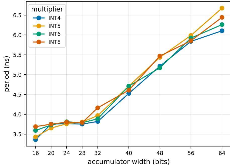
smallest valid achieved period
