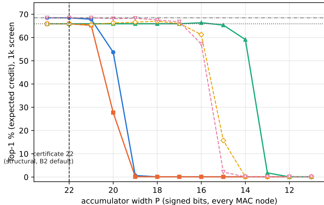
ResNet18 INT6
