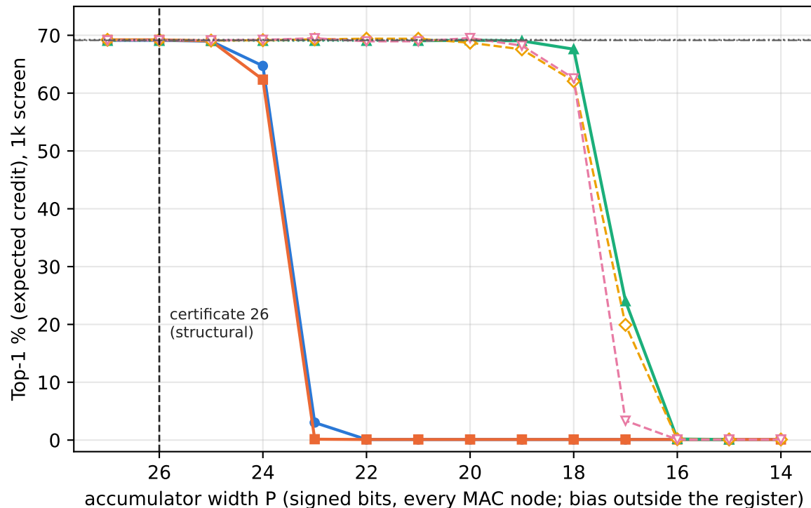
ResNet18 INT8
