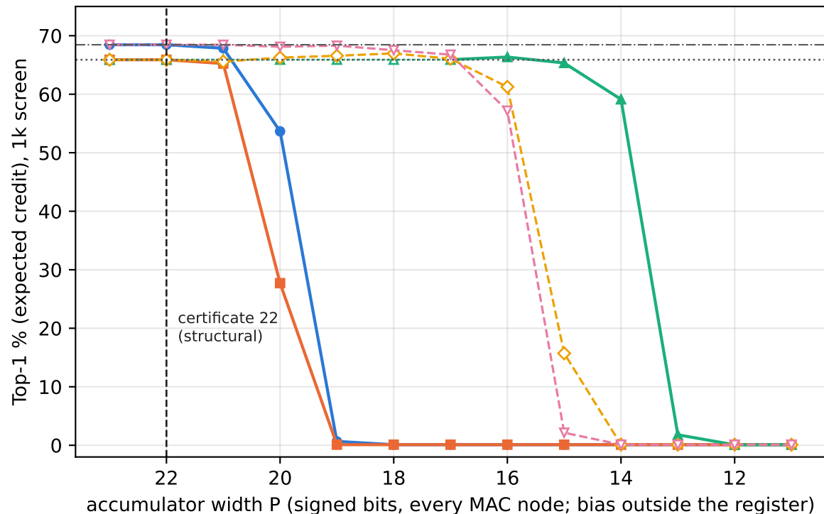
ResNet18 INT6
