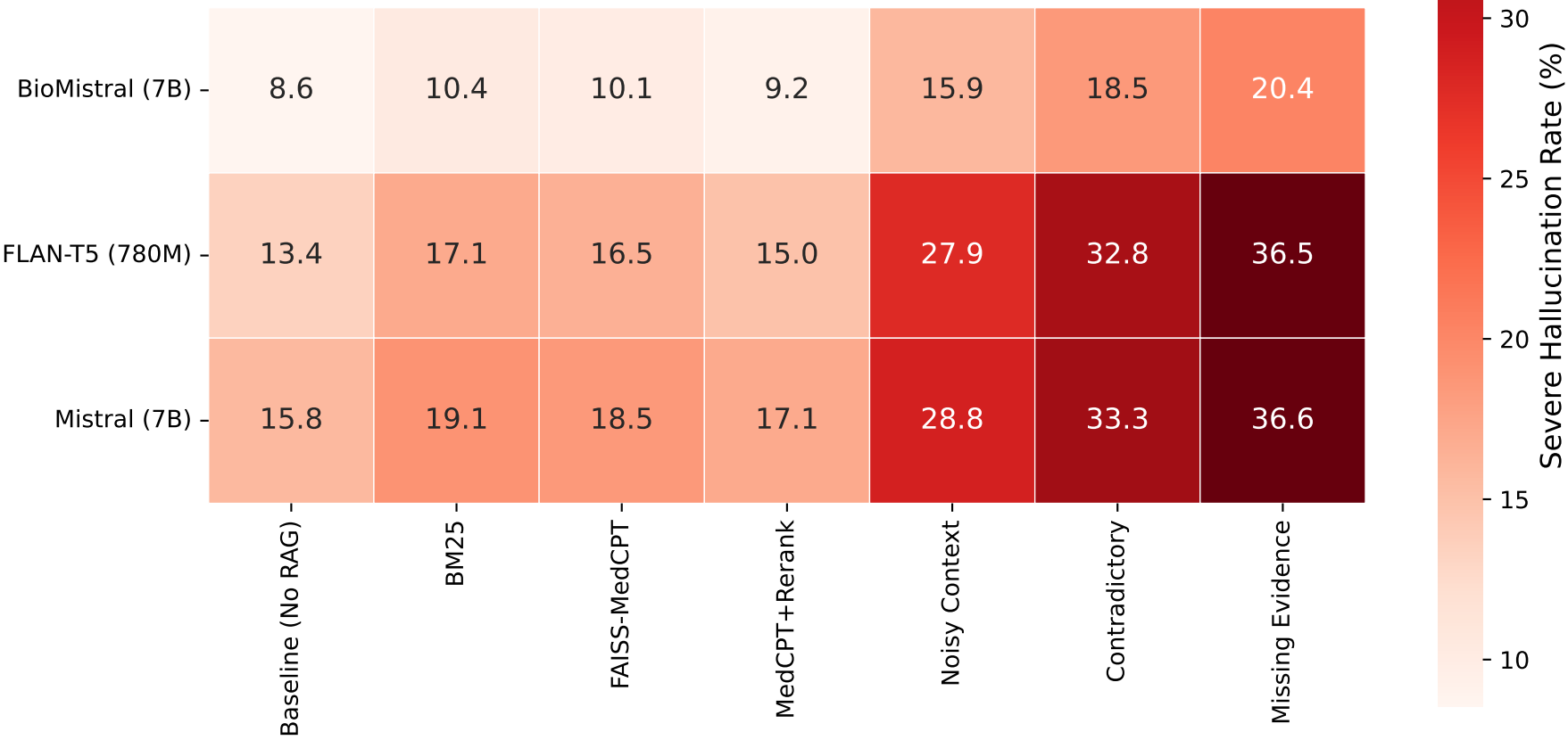
Severe Hallucination Rate Across Models and RAG Conditions
