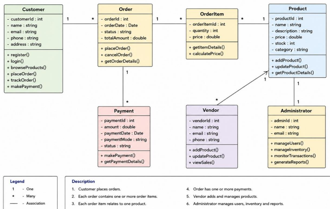
Figure 3: Online Retail Shopping Platform – Class Diagram
