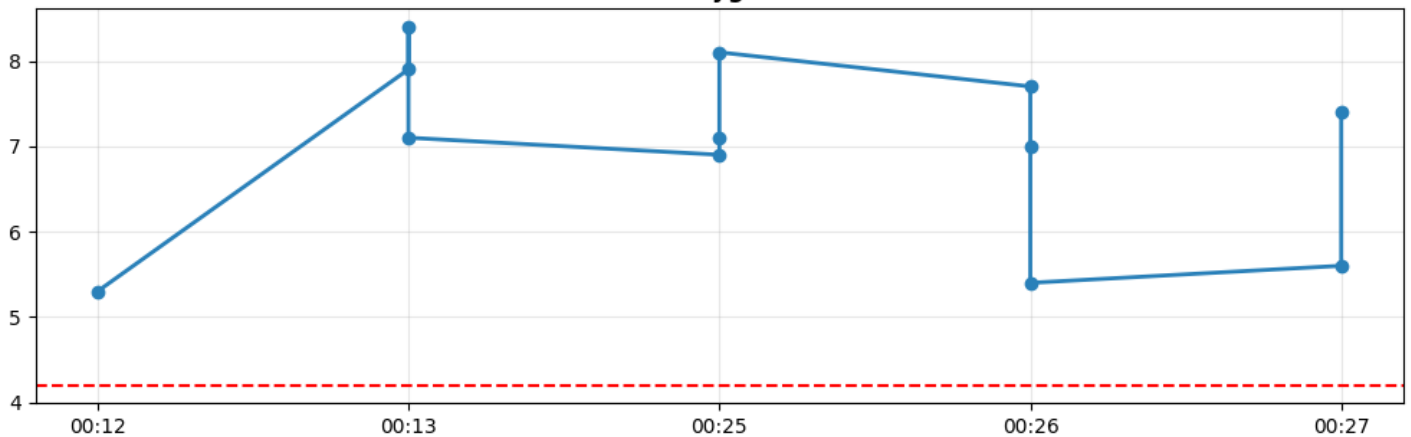
Dissolved Oxygen (Pond 3)
