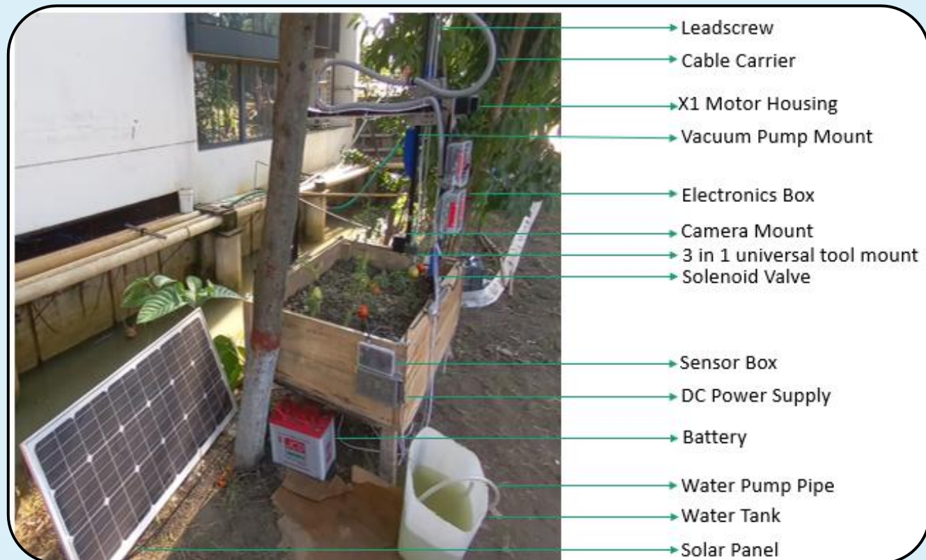
System Setup for Farmbot on Farming Bed
