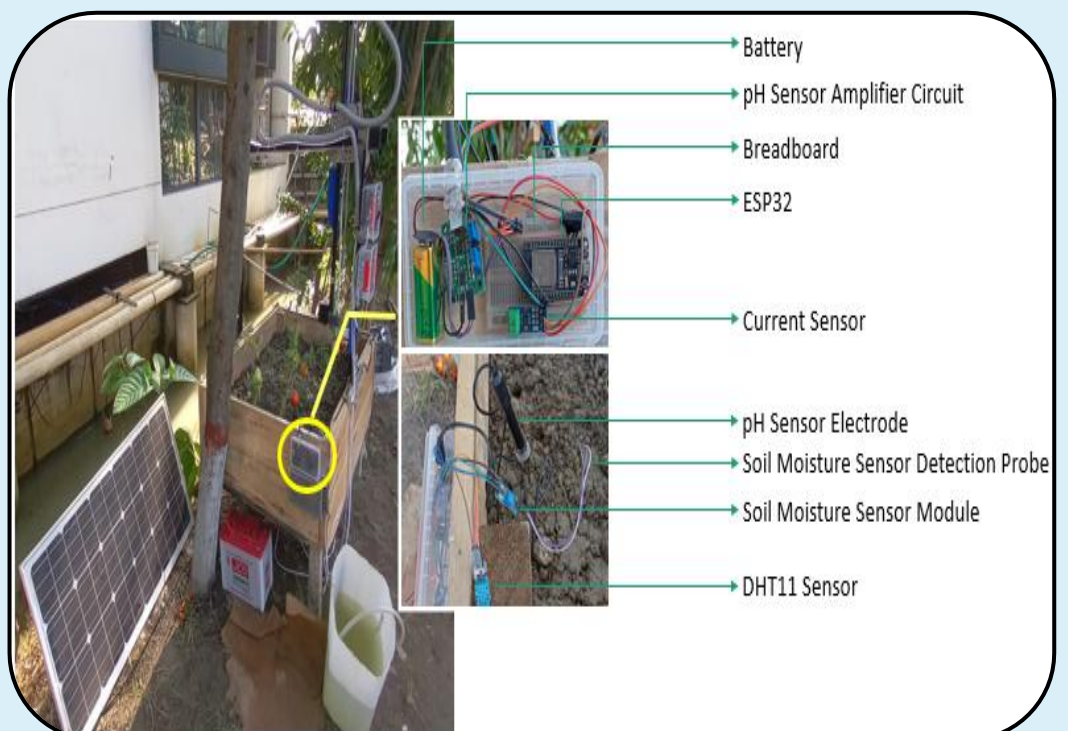
Farmbot and Sensor Box Setup
