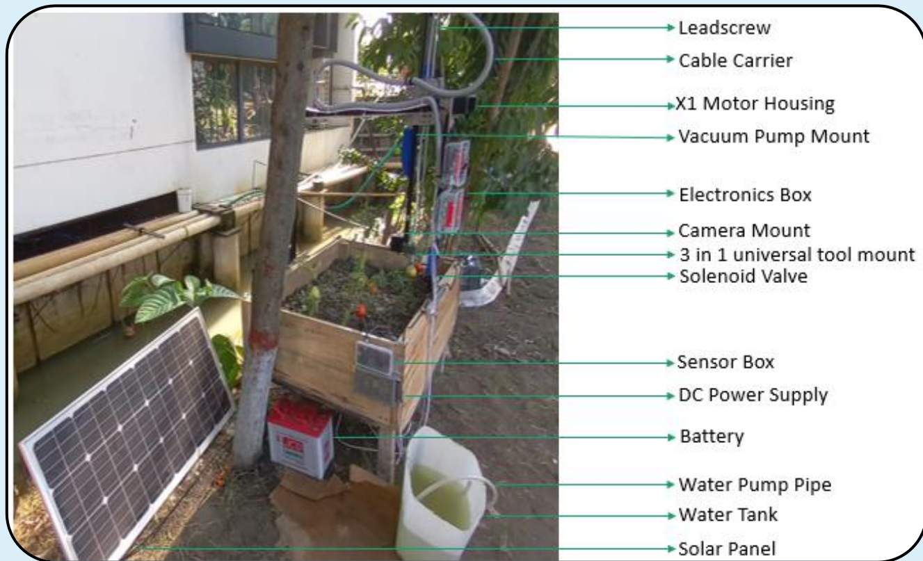
System Setup for Farmbot on Farming Bed
