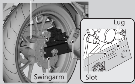
Brake caliper bracket
