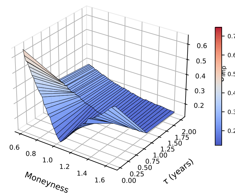
Historical: Forecast
