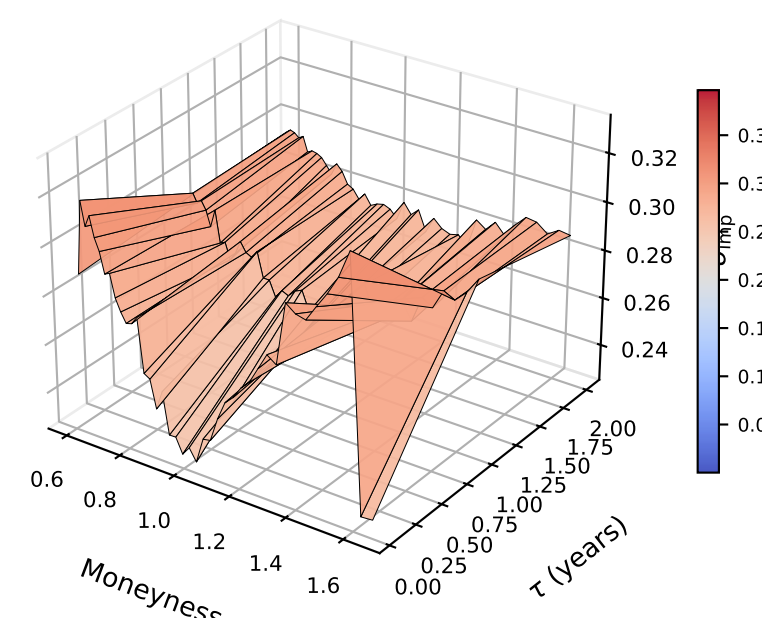
Heston: Forecast
