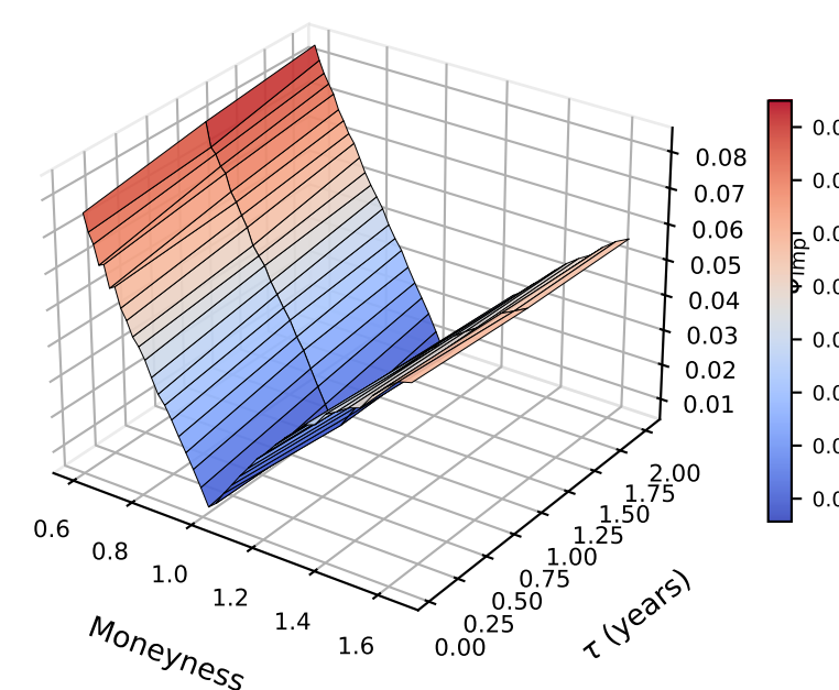
Sabr: Forecast
