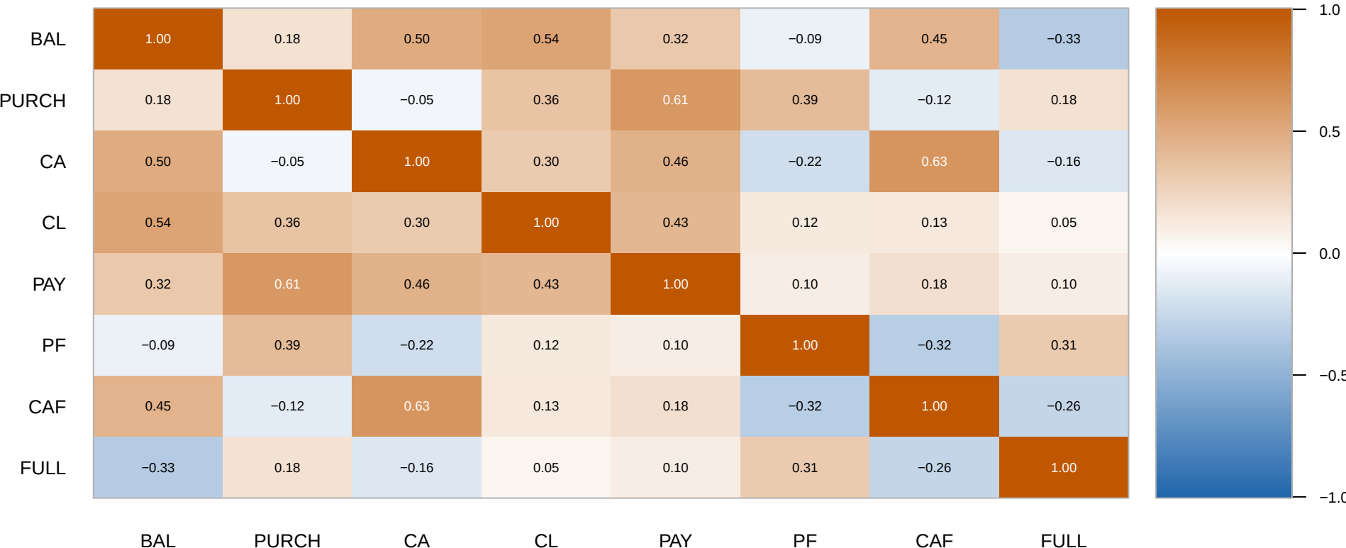
Correlation Matrix -- Clustering Variables
