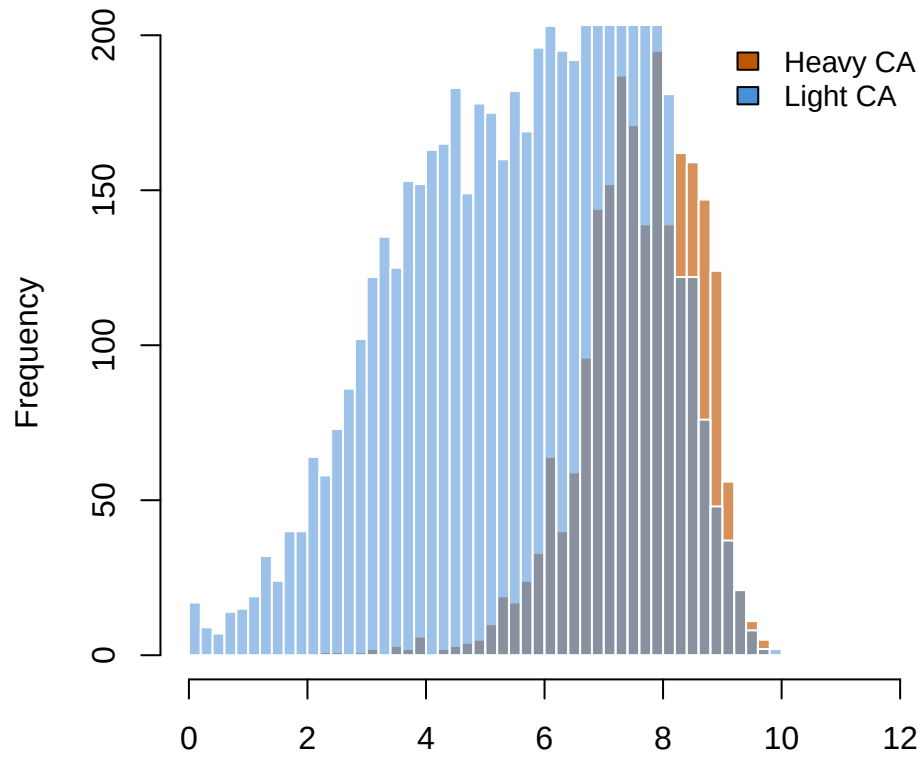
Log-Balance Distribution
