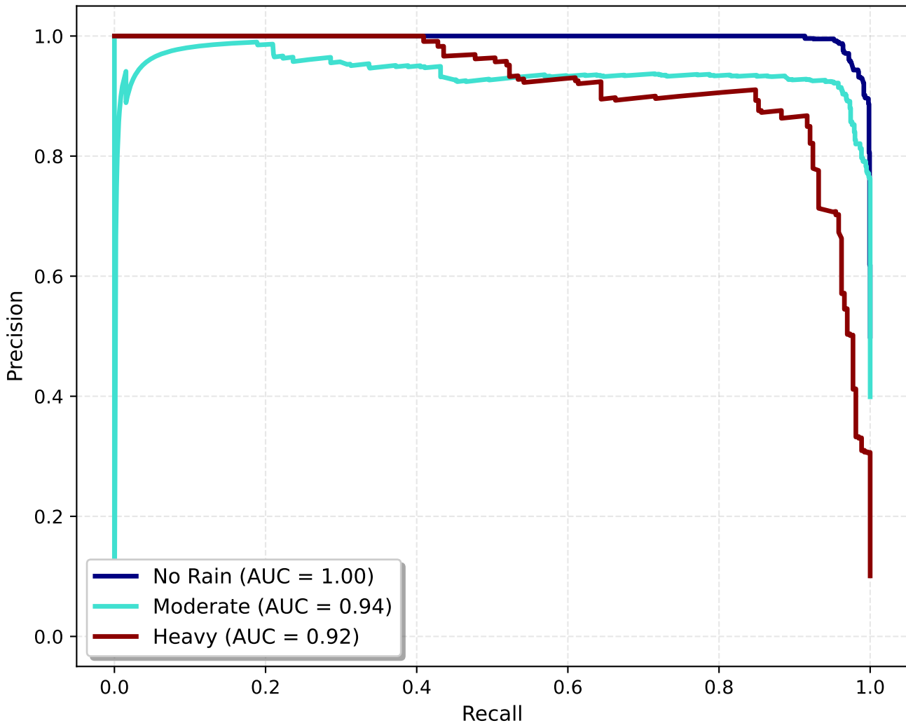
Precision-Recall Curve: XGB Champion
