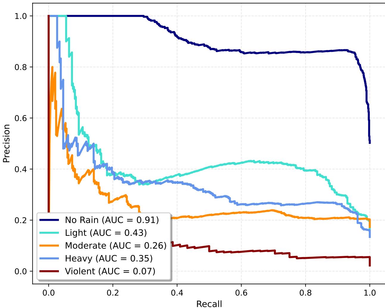
Precision-Recall Curve: NUSVC Champion
