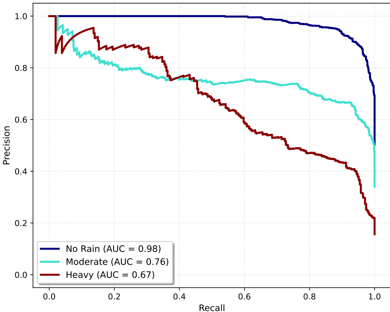
Precision-Recall Curve: RF Champion
