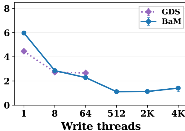
Post-write Read BW (GiB/s)
