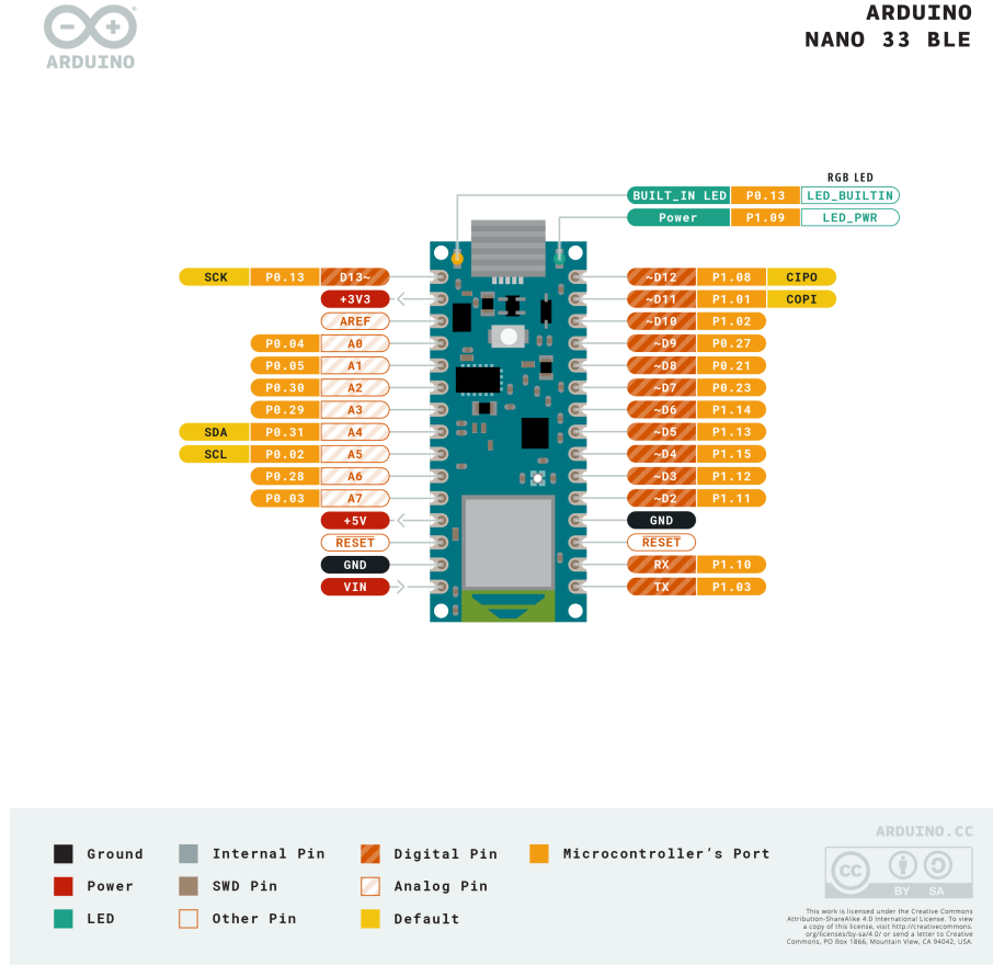
Figure 3.2: Arduino Nano BLE Rev 2 - Pinout[3]
