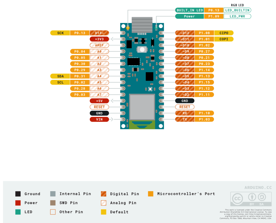
Figure 3.3: Arduino Nano BLE Rev 2 - Pinout[4]
