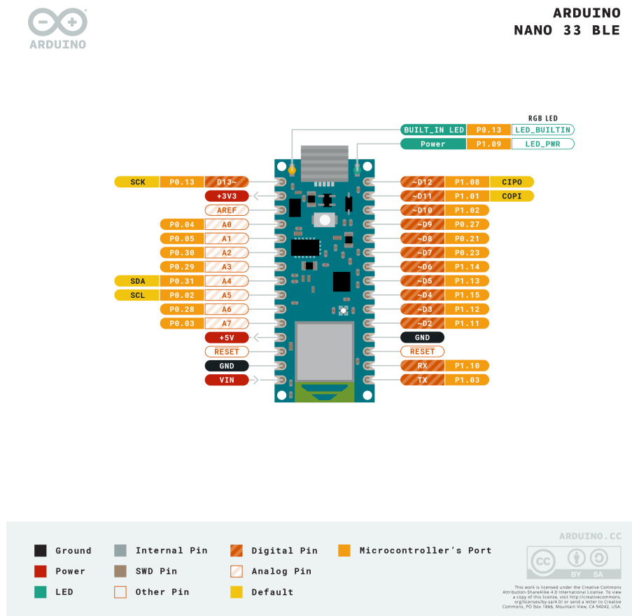
Figure 3.3: Arduino Nano BLE Rev 2 - Pinout[3]
