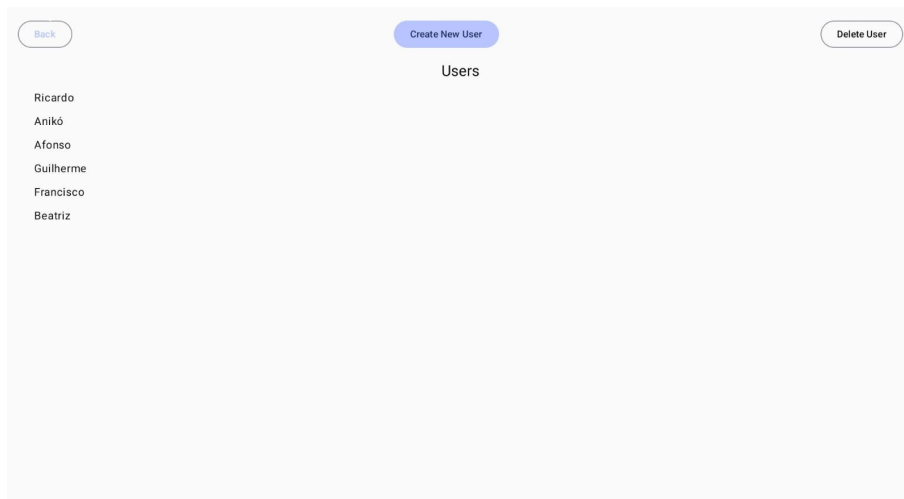
Figure 4.3: Profiles' Menu
