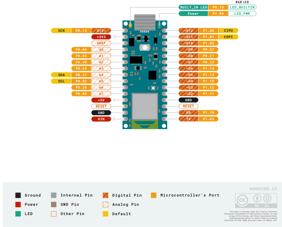
Figure 3.2: Arduino Nano BLE Rev 2 - Pinout[3]
