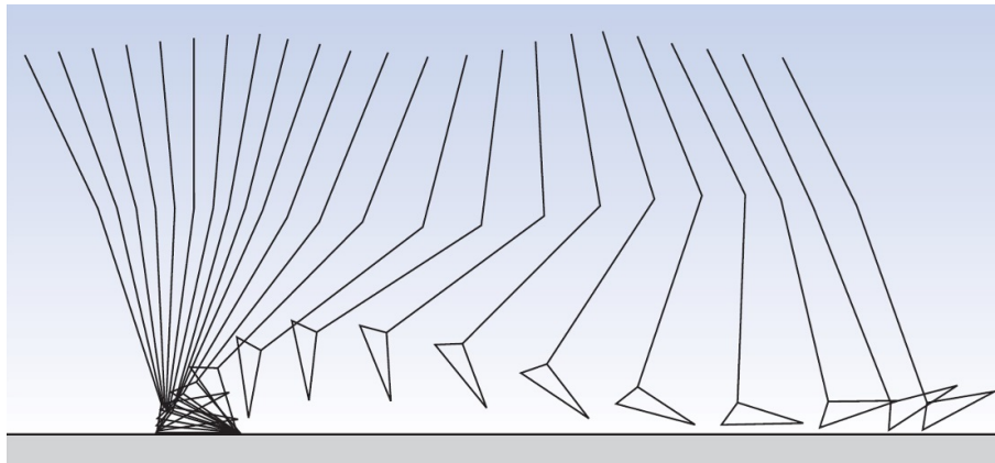
Figure 2.1: The gait cycle of a leg with with a cycle time of 0.92s. 40 ms interval between lines [13].
