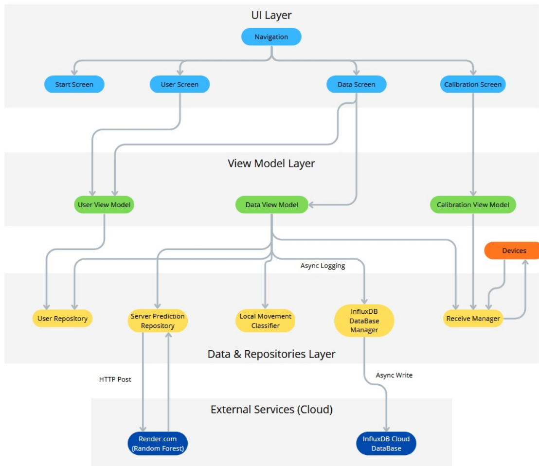
Figure 4.1: Android Application Overview
