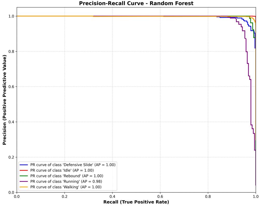
Figure 5.6: RF Precision Recall Curve
