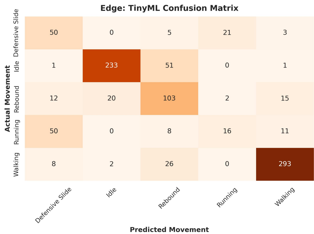
Figure 5.13: Confusion Matrix for the TinyML Model
