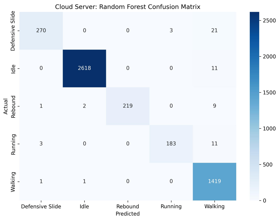
Figure 5.9: Random ForestL Confusion Matrix
