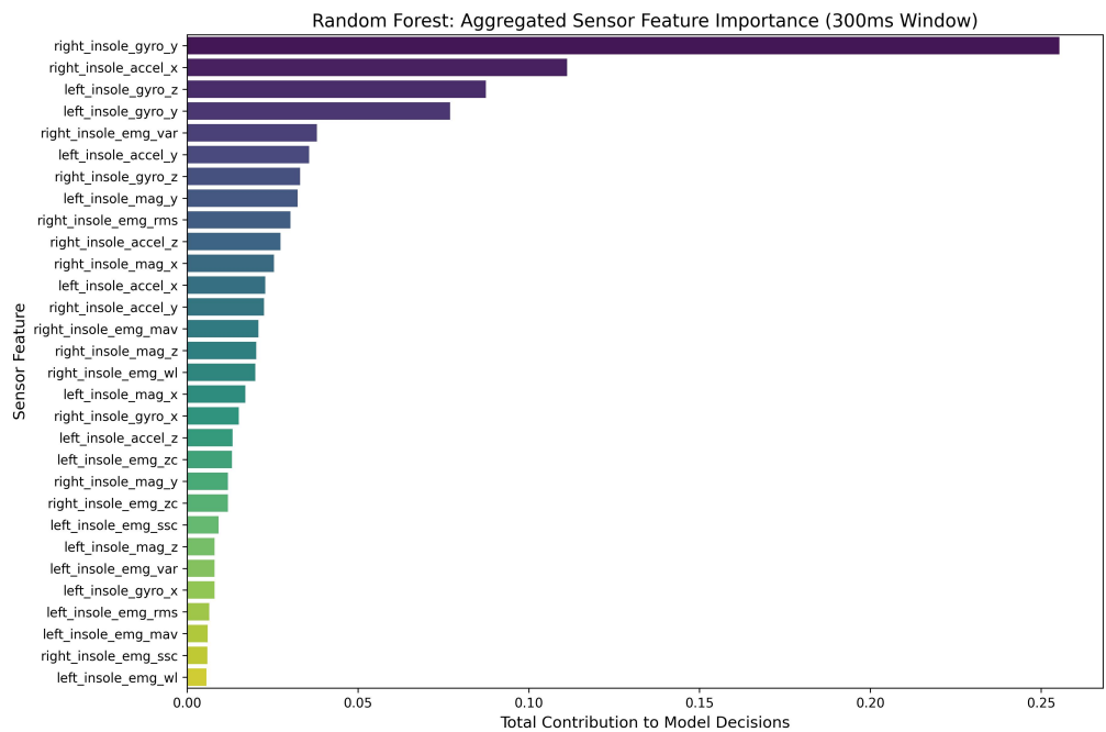
Figure 5.7: Feature Importance Graph
