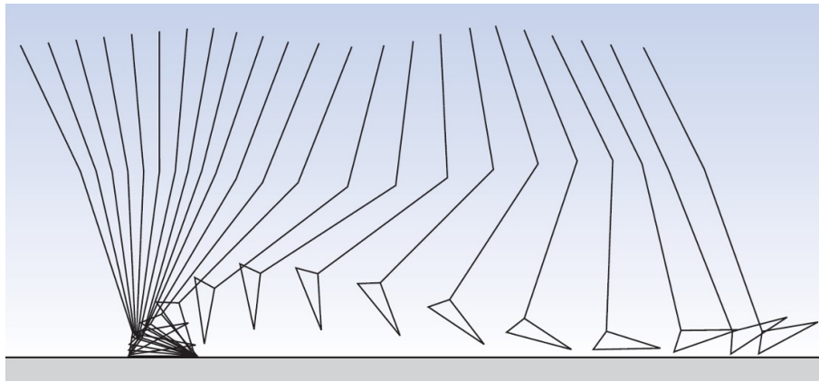
Figure 2.1: The gait cycle of a leg with with a cycle time of 0.92s. 40 ms interval between lines [20].
