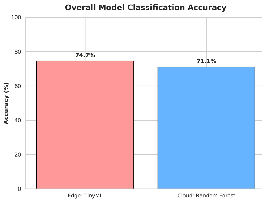
Figure 5.10: Overall Classification Accuracy: Local TinyML vs. Cloud Random Forest
