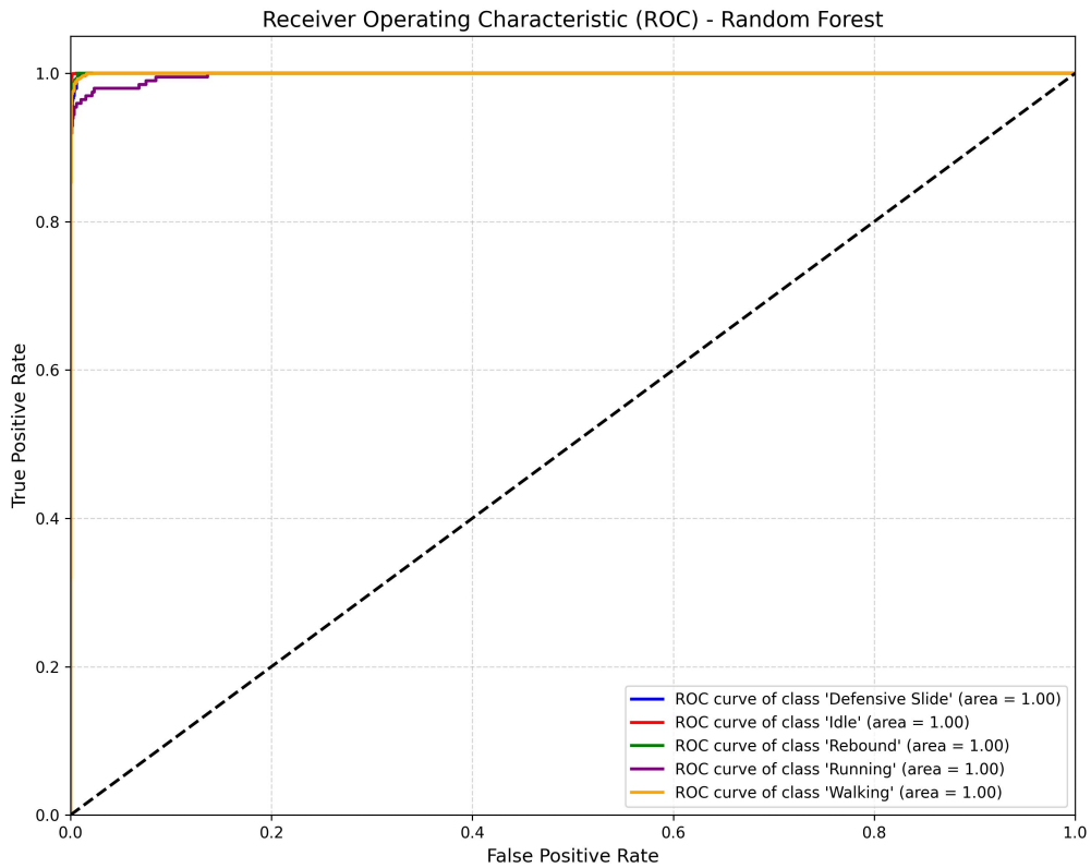
Figure 5.5: RF ROC Curve
