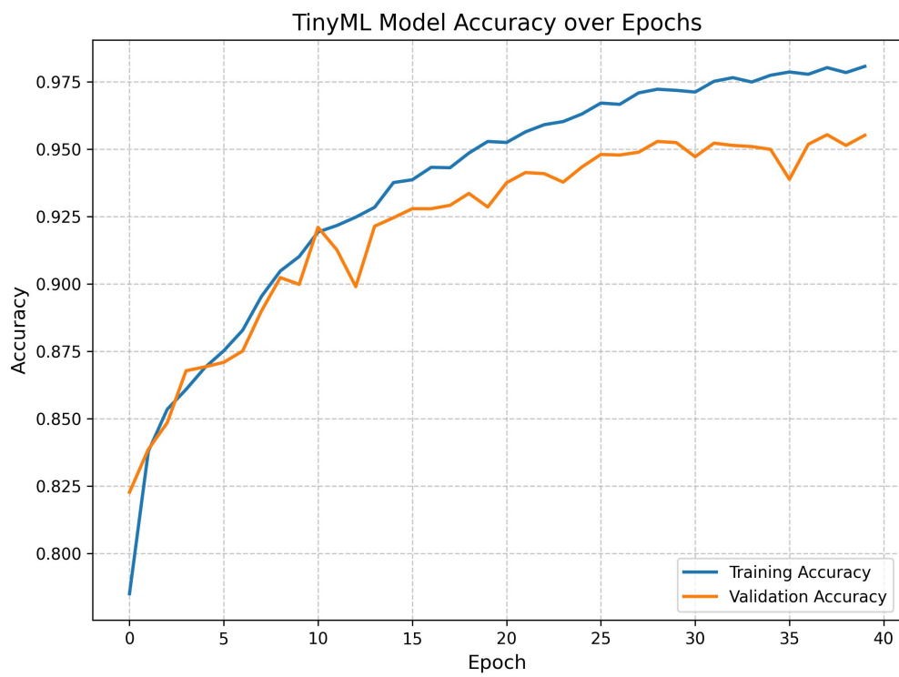
Figure 5.3: TinyMLAccuracy
