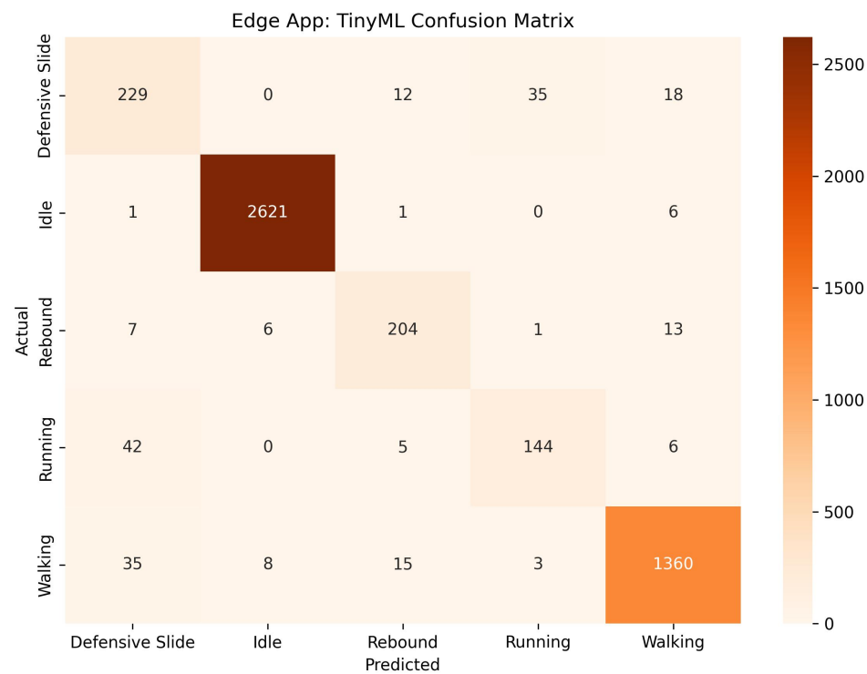
Figure 5.8: TinyML Confusion Matrix
