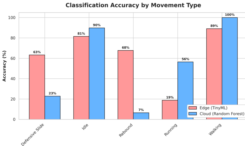
Figure 5.11: Classification Accuracy by Movement
