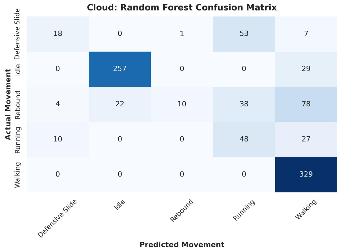
Figure 5.12: Confusion Matrix for the Random Forest Model
