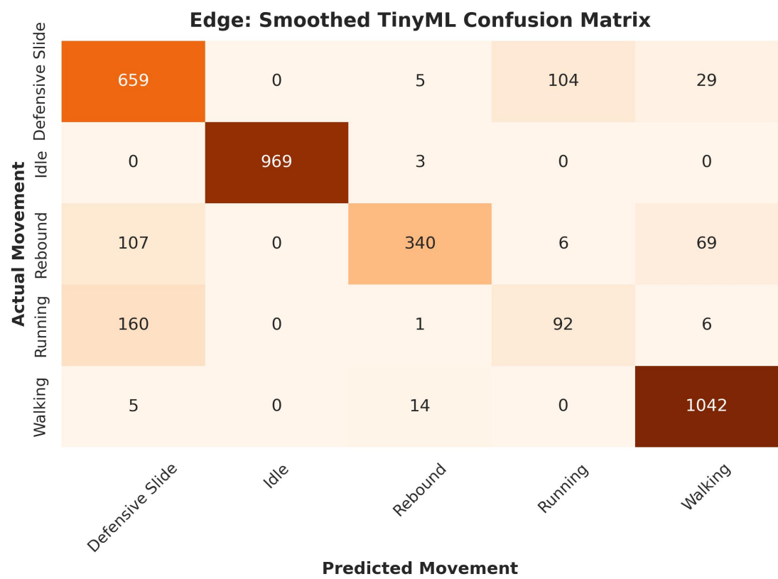
Figure 5.15: Confusion Matrix for the Smoothed TinyML Model
