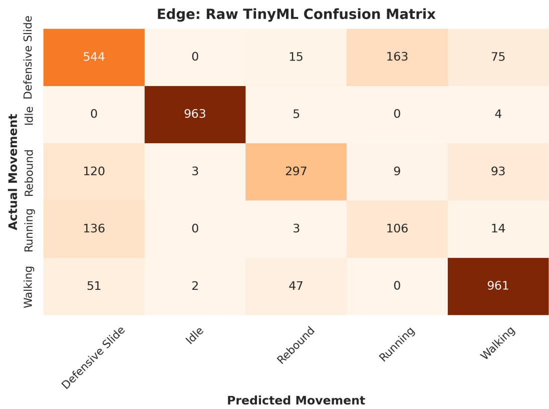
Figure 5.14: Confusion Matrix for the Raw TinyML Model
