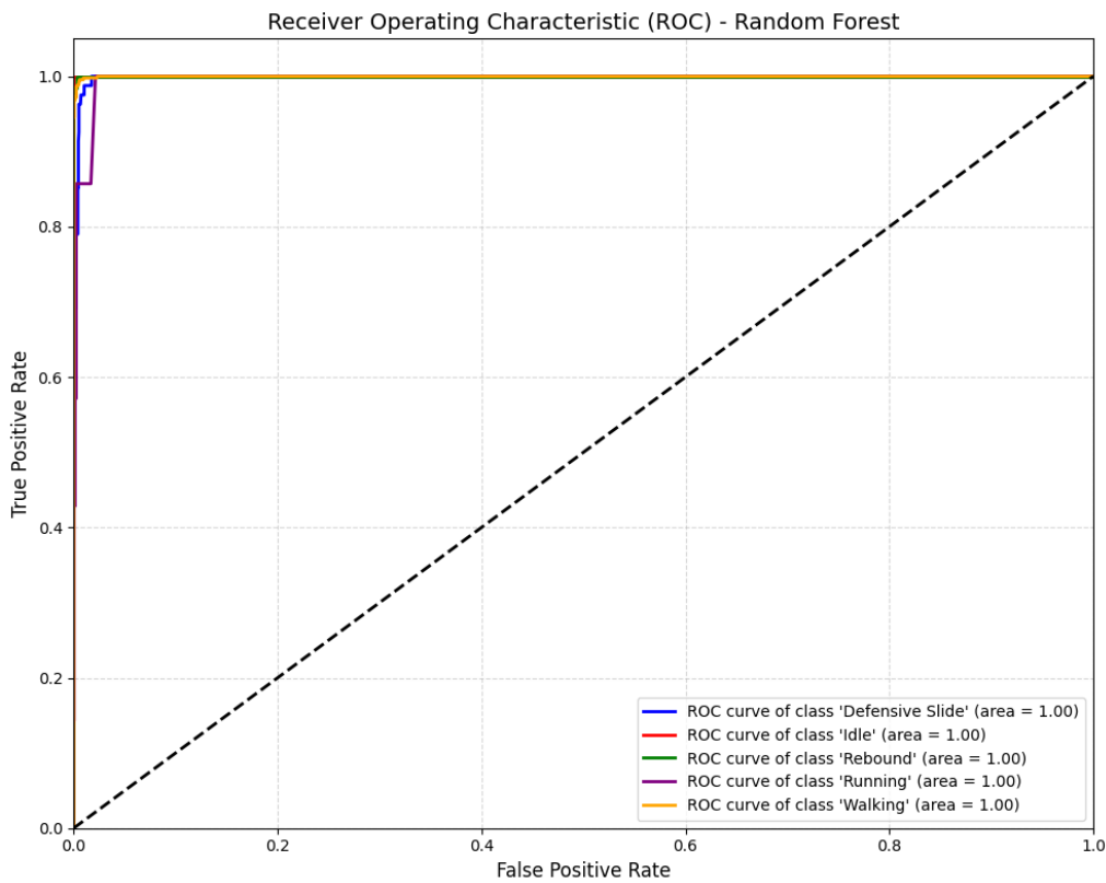
Figure 5.8: RF ROC Curve
