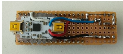
(b) Bottom side - EMG sensor
