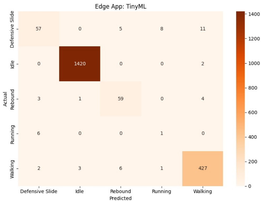
Figure 5.6: TinyML Confusion Matrix
