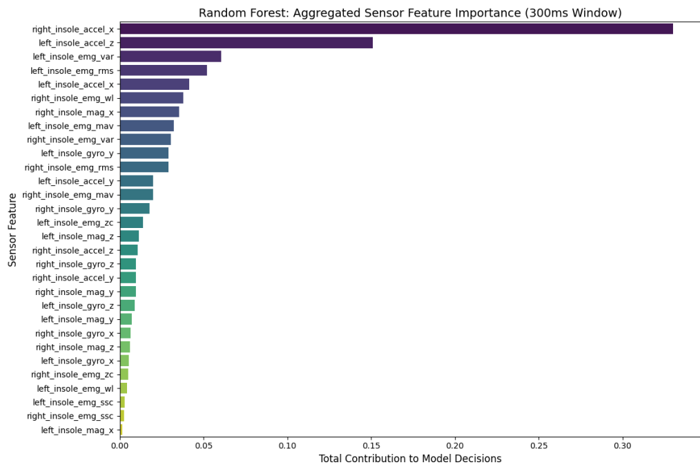
Figure 5.5: Feature Importance Graph
