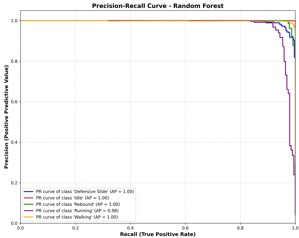
Figure 5.9: RF Precision Recall Curve
