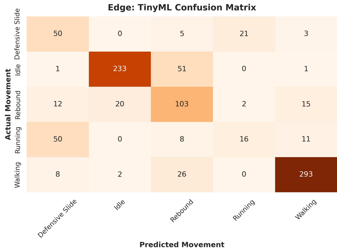
Figure 5.13: Confusion Matrix for the TinyML Model
