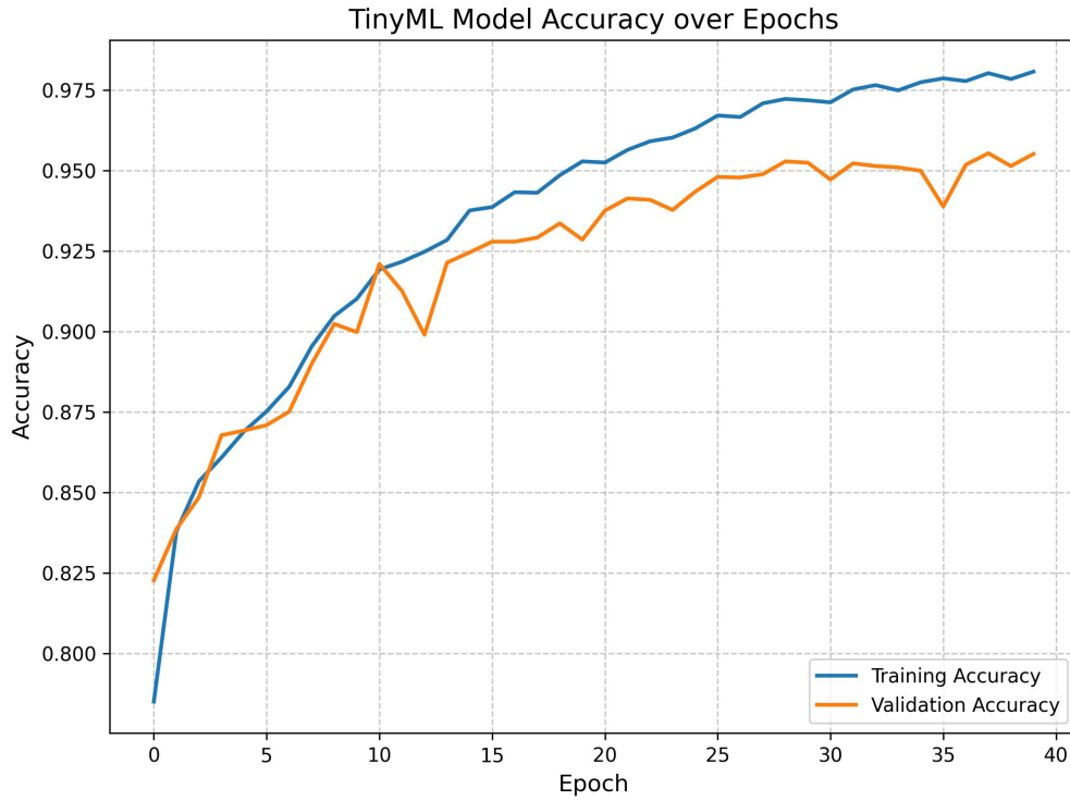
Figure 5.3: TinyMLAccuracy
