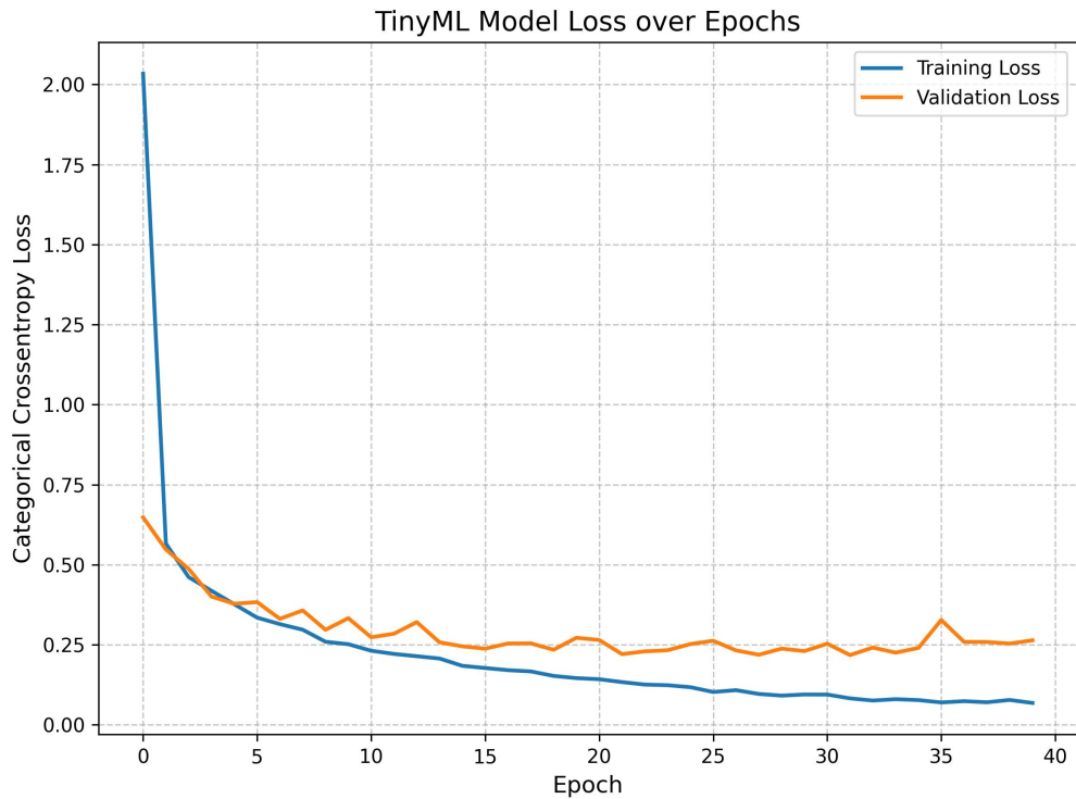
Figure 5.4: TinyMLLoss
