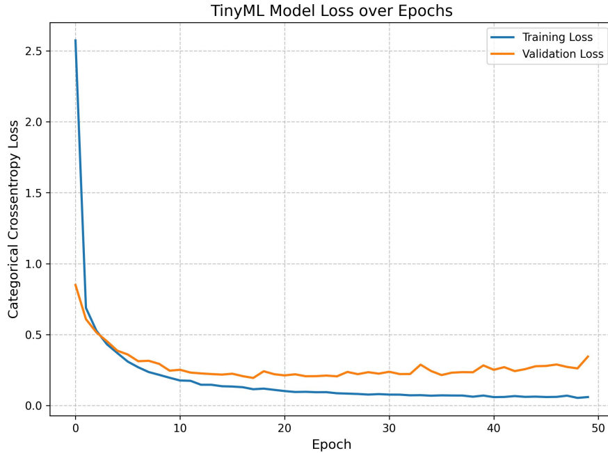
Figure 5.4: TinyMLLoss
