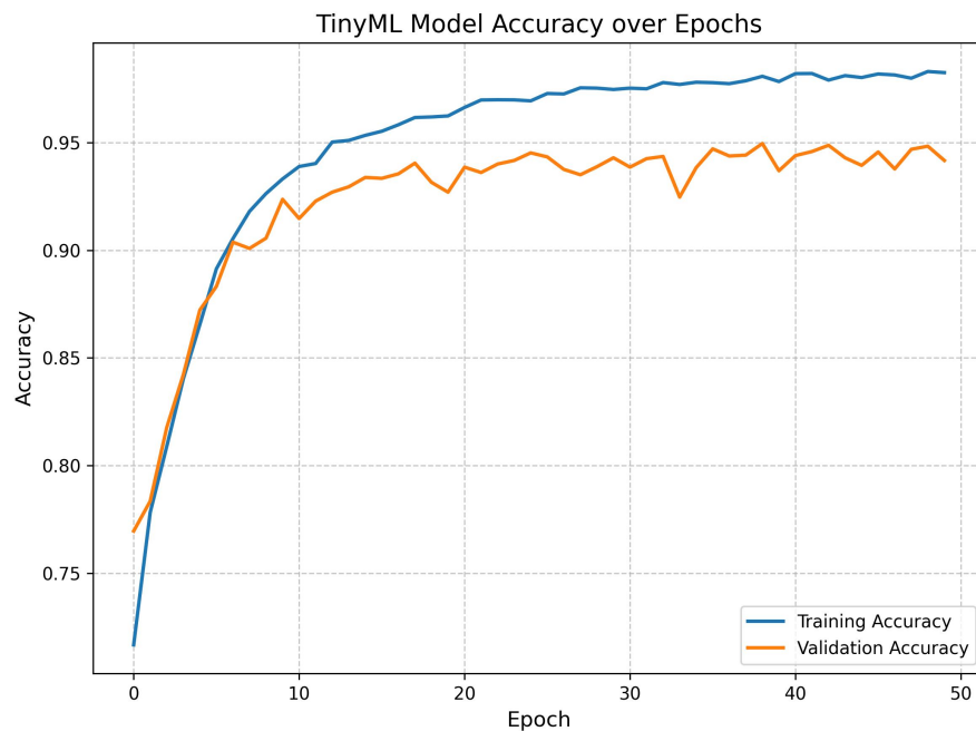
Figure 5.3: TinyMLAccuracy
